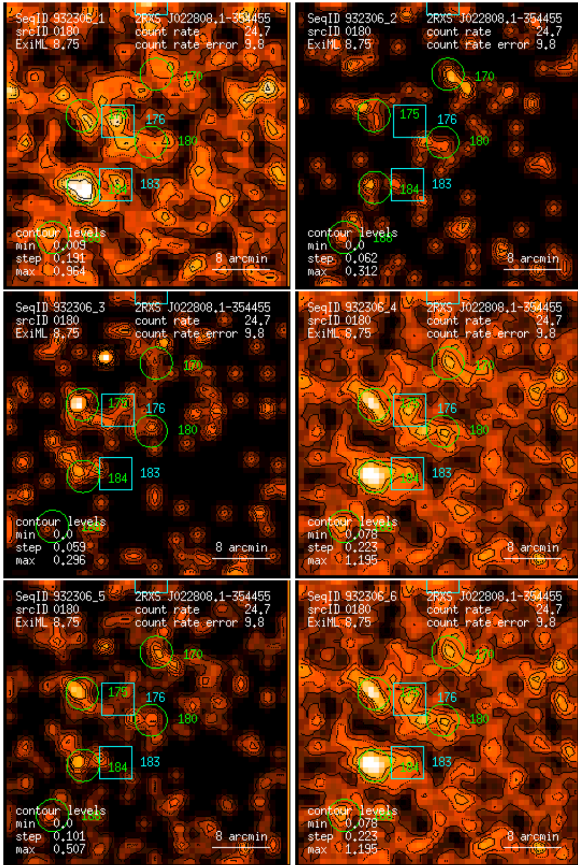
Figure 180: RASS 932306: detection 0180: band rate images, Gaussian filter: (1) PSPC channels 11 – 41, (2) 52 – 90, (3) 91 – 201, (4) 11 – 235, (5) 52 – 201, (6) 11 – 201. Broad band rates in counts/ks. Band rate contour levels in counts/ks/arcmin 2 .
