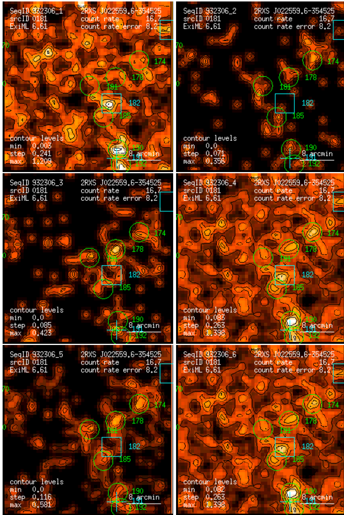
Figure 181: RASS 932306: detection 0181: band rate images, Gaussian filter: (1) PSPC channels 11 – 41, (2) 52 – 90, (3) 91 – 201, (4) 11 – 235, (5) 52 – 201, (6) 11 – 201. Broad band rates in counts/ks. Band rate contour levels in counts/ks/arcmin 2 .
