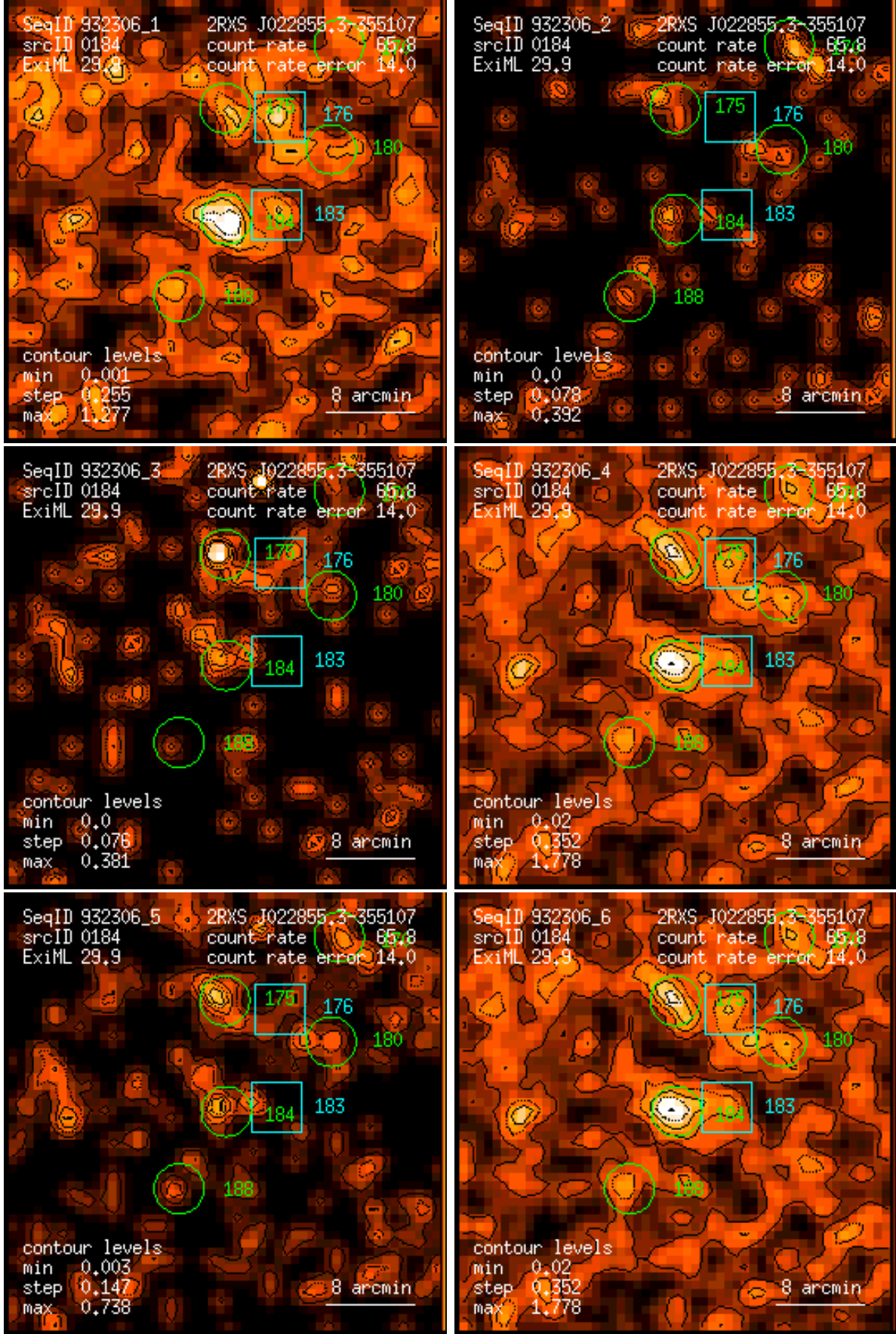
Figure 184: RASS 932306: detection 0184: band rate images, Gaussian filter: (1) PSPC channels 11 – 41, (2) 52 – 90, (3) 91 – 201, (4) 11 – 235, (5) 52 – 201, (6) 11 – 201. Broad band rates in counts/ks. Band rate contour levels in counts/ks/arcmin 2 .
