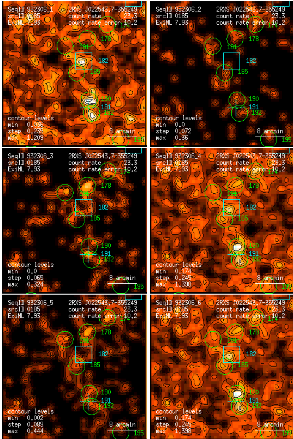
Figure 185: RASS 932306: detection 0185: band rate images, Gaussian filter: (1) PSPC channels 11 – 41, (2) 52 – 90, (3) 91 – 201, (4) 11 – 235, (5) 52 – 201, (6) 11 – 201. Broad band rates in counts/ks. Band rate contour levels in counts/ks/arcmin 2 .
