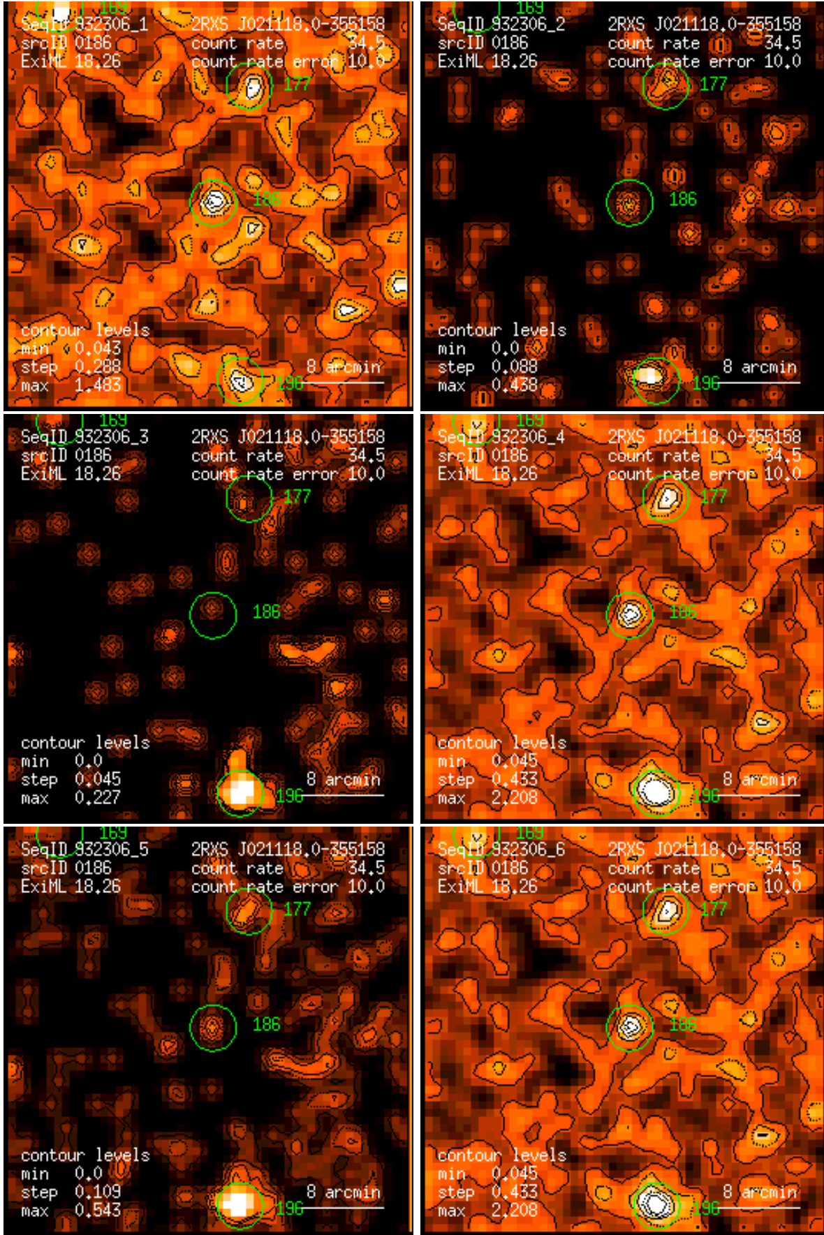
Figure 186: RASS 932306: detection 0186: band rate images, Gaussian filter: (1) PSPC channels 11 – 41, (2) 52 – 90, (3) 91 – 201, (4) 11 – 235, (5) 52 – 201, (6) 11 – 201. Broad band rates in counts/ks. Band rate contour levels in counts/ks/arcmin 2 .
