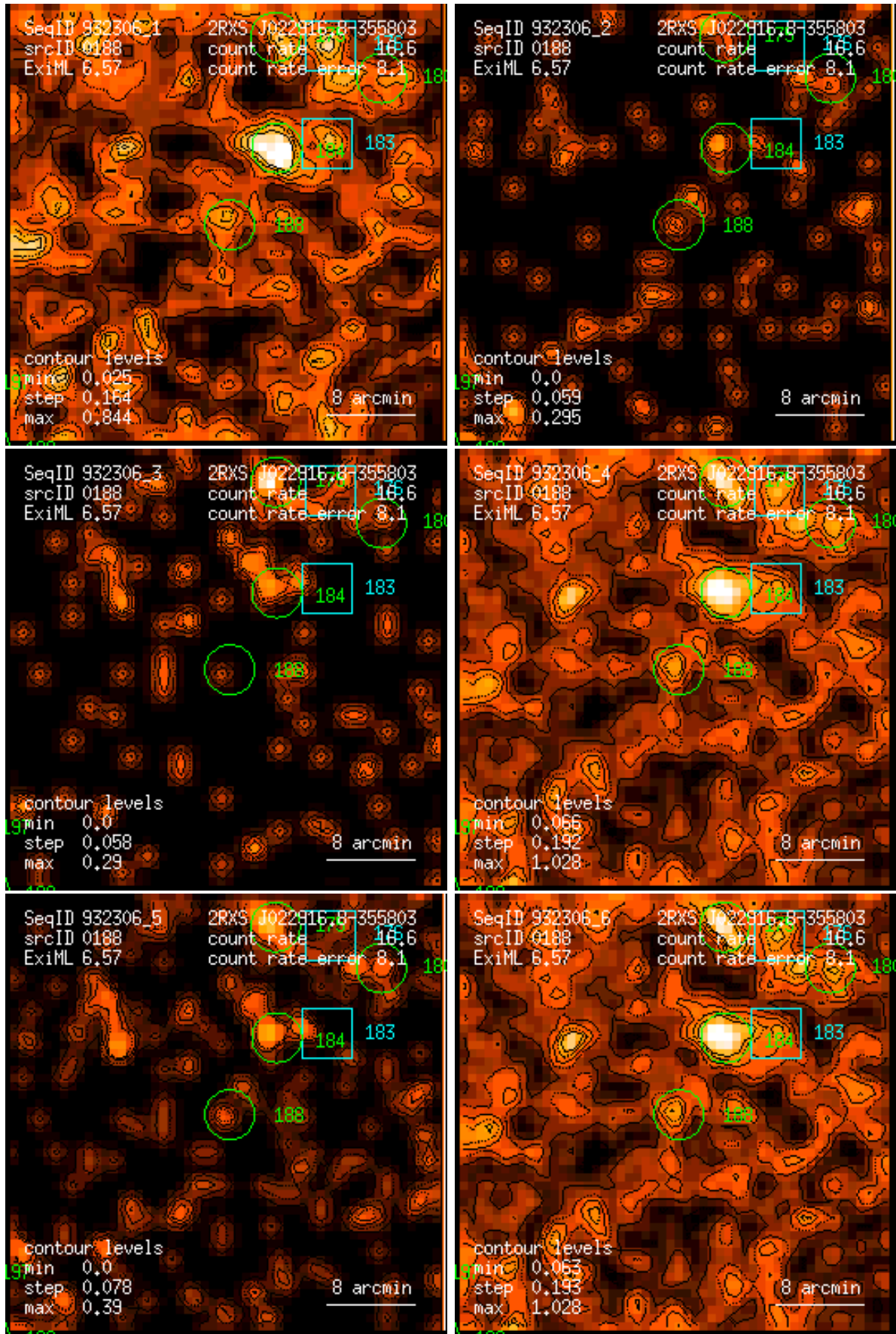
Figure 188: RASS 932306: detection 0188: band rate images, Gaussian filter: (1) PSPC channels 11 – 41, (2) 52 – 90, (3) 91 – 201, (4) 11 – 235, (5) 52 – 201, (6) 11 – 201. Broad band rates in counts/ks. Band rate contour levels in counts/ks/arcmin 2 .
