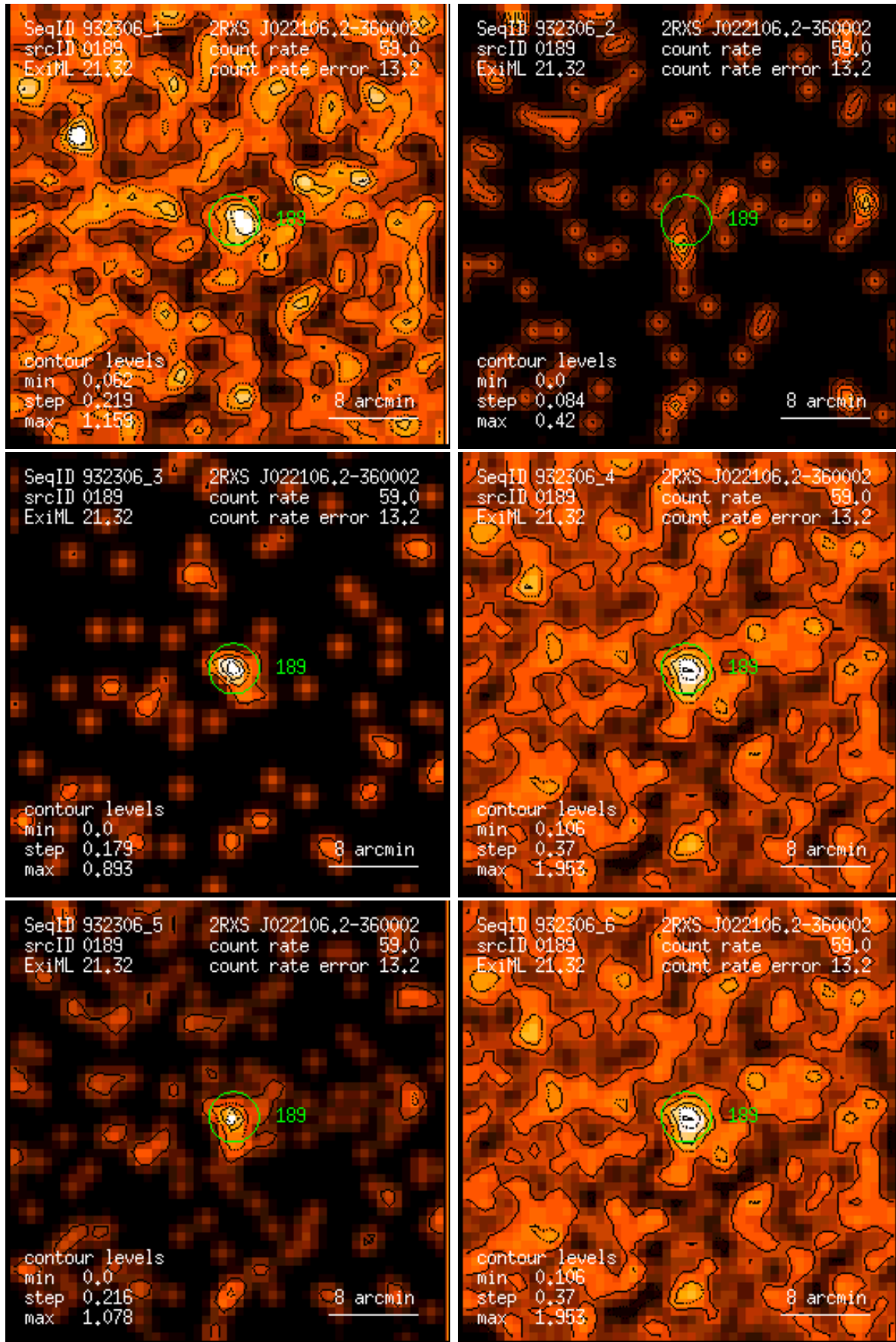
Figure 189: RASS 932306: detection 0189: band rate images, Gaussian filter: (1) PSPC channels 11 – 41, (2) 52 – 90, (3) 91 – 201, (4) 11 – 235, (5) 52 – 201, (6) 11 – 201. Broad band rates in counts/ks. Band rate contour levels in counts/ks/arcmin 2 .
