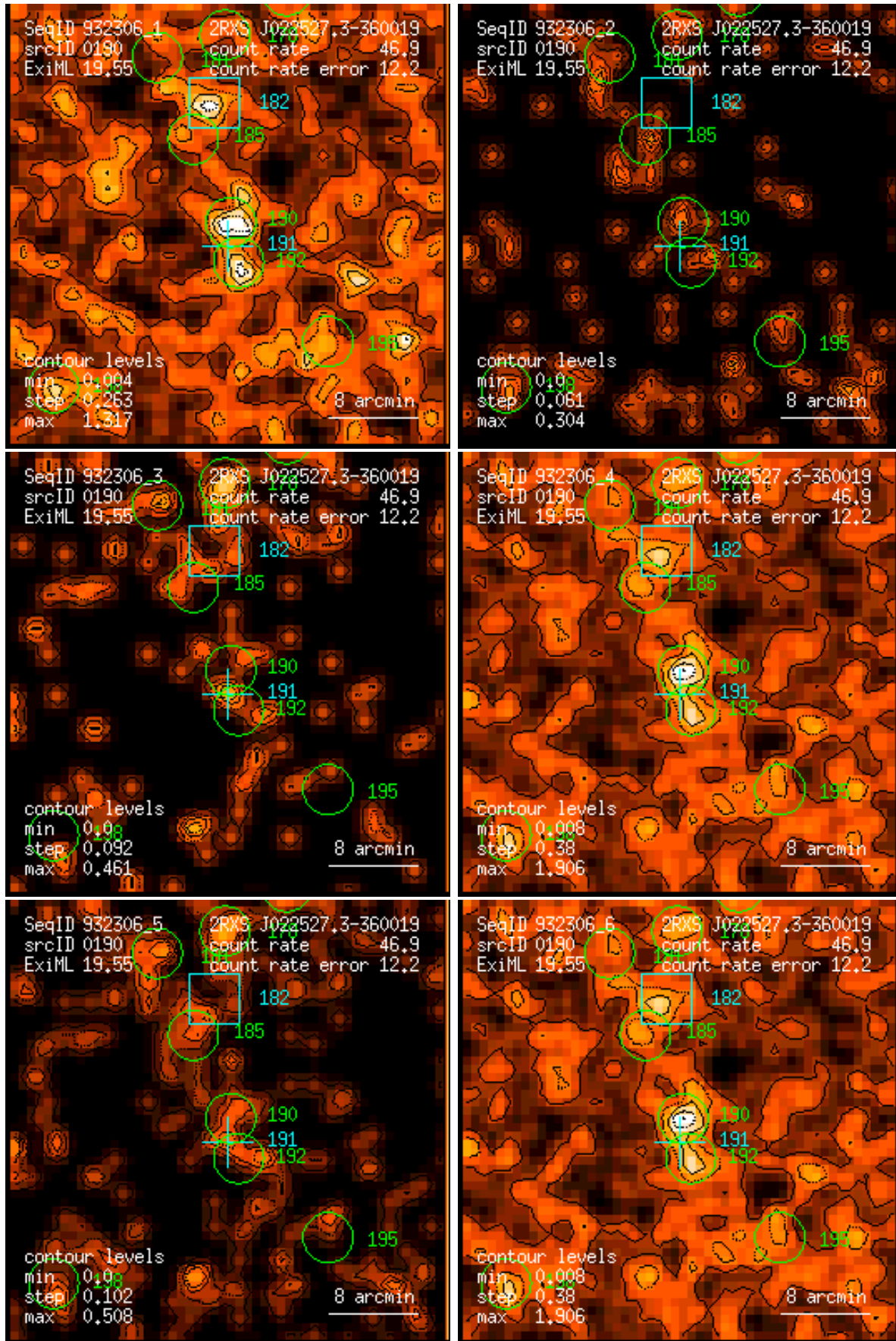
Figure 190: RASS 932306: detection 0190: band rate images, Gaussian filter: (1) PSPC channels 11 – 41, (2) 52 – 90, (3) 91 – 201, (4) 11 – 235, (5) 52 – 201, (6) 11 – 201. Broad band rates in counts/ks. Band rate contour levels in counts/ks/arcmin 2 .
