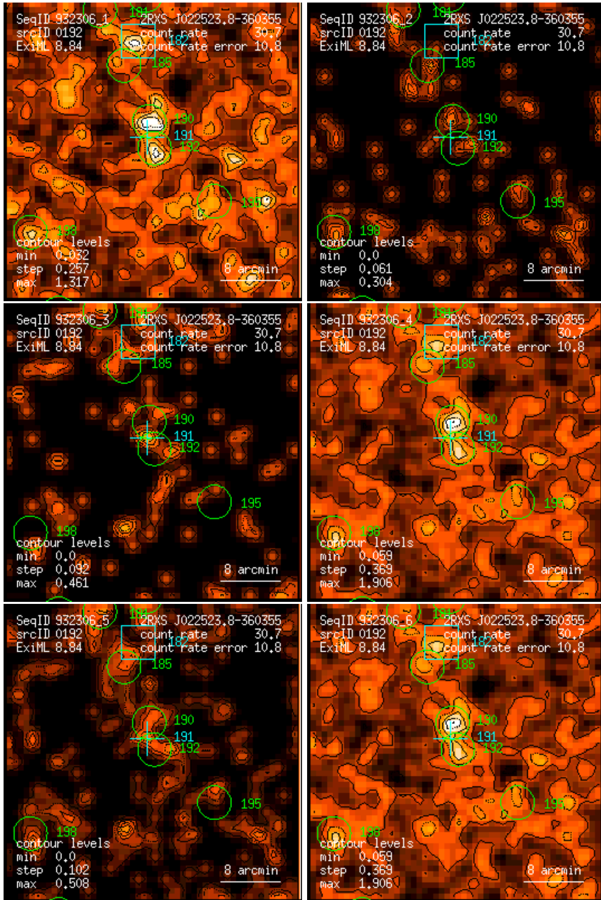
Figure 192: RASS 932306: detection 0192: band rate images, Gaussian filter: (1) PSPC channels 11 – 41, (2) 52 – 90, (3) 91 – 201, (4) 11 – 235, (5) 52 – 201, (6) 11 – 201. Broad band rates in counts/ks. Band rate contour levels in counts/ks/arcmin 2 .
