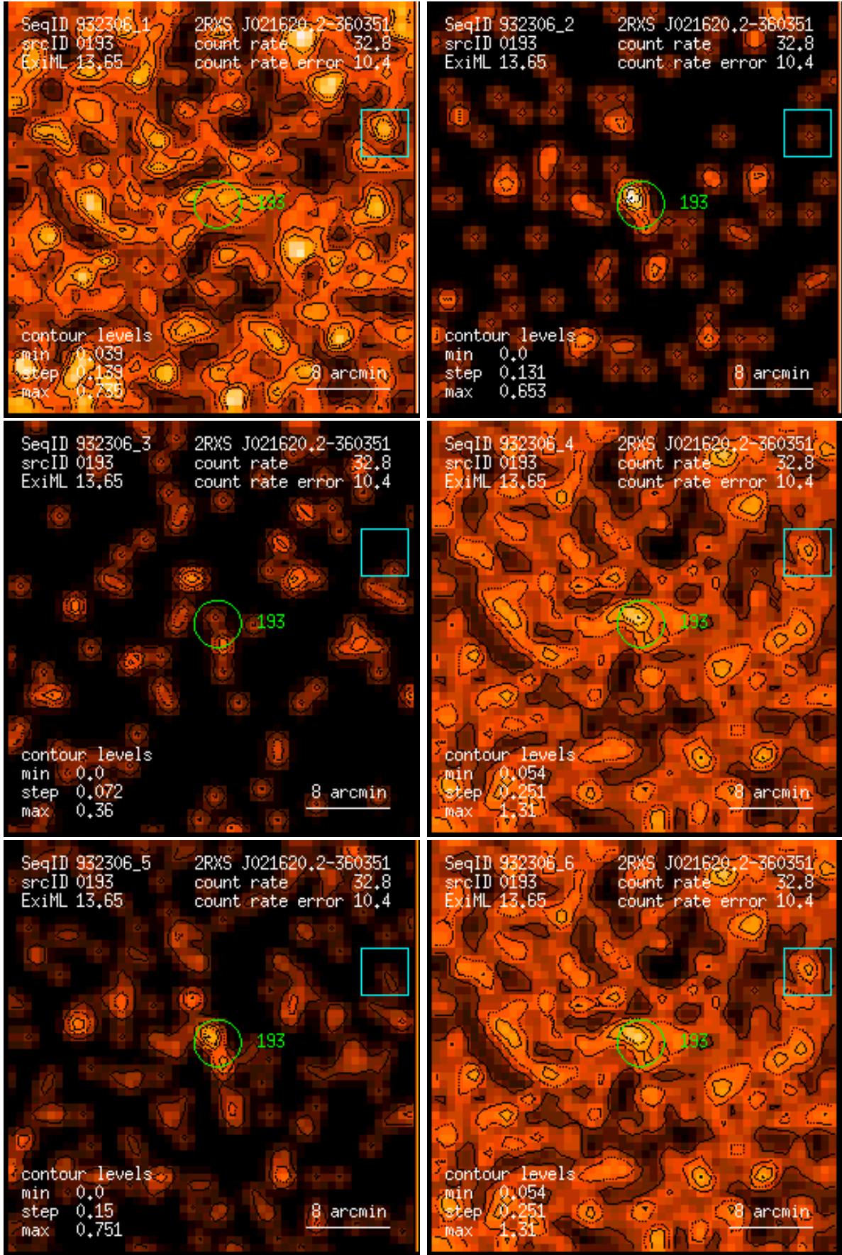
Figure 193: RASS 932306: detection 0193: band rate images, Gaussian filter: (1) PSPC channels 11 – 41, (2) 52 – 90, (3) 91 – 201, (4) 11 – 235, (5) 52 – 201, (6) 11 – 201. Broad band rates in counts/ks. Band rate contour levels in counts/ks/arcmin 2 .
