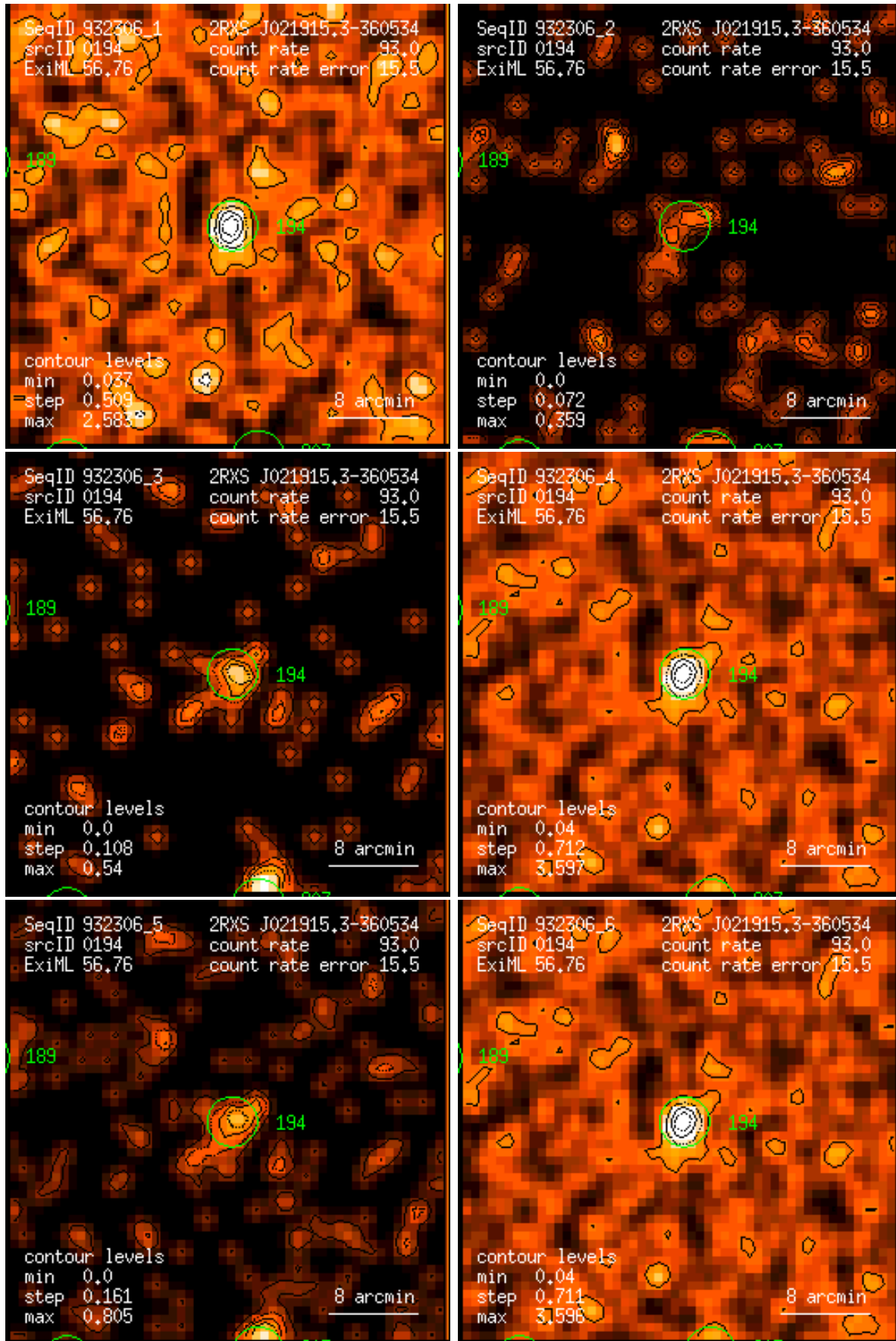
Figure 194: RASS 932306: detection 0194: band rate images, Gaussian filter: (1) PSPC channels 11 – 41, (2) 52 – 90, (3) 91 – 201, (4) 11 – 235, (5) 52 – 201, (6) 11 – 201. Broad band rates in counts/ks. Band rate contour levels in counts/ks/arcmin 2 .
