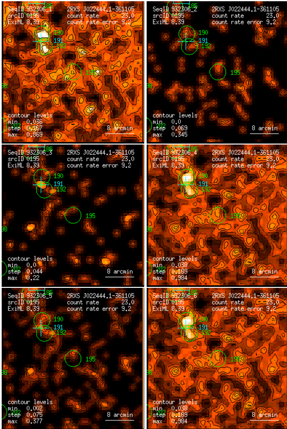
Figure 195: RASS 932306: detection 0195: band rate images, Gaussian filter: (1) PSPC channels 11 – 41, (2) 52 – 90, (3) 91 – 201, (4) 11 – 235, (5) 52 – 201, (6) 11 – 201. Broad band rates in counts/ks. Band rate contour levels in counts/ks/arcmin 2 .
