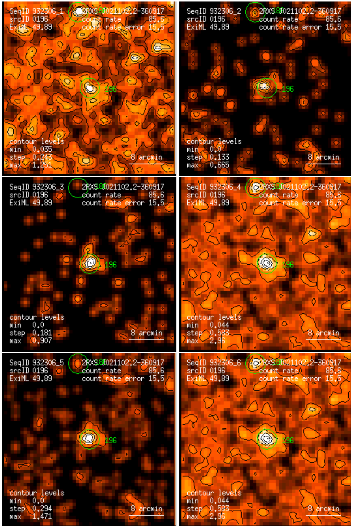
Figure 196: RASS 932306: detection 0196: band rate images, Gaussian filter: (1) PSPC channels 11 – 41, (2) 52 – 90, (3) 91 – 201, (4) 11 – 235, (5) 52 – 201, (6) 11 – 201. Broad band rates in counts/ks. Band rate contour levels in counts/ks/arcmin 2 .
