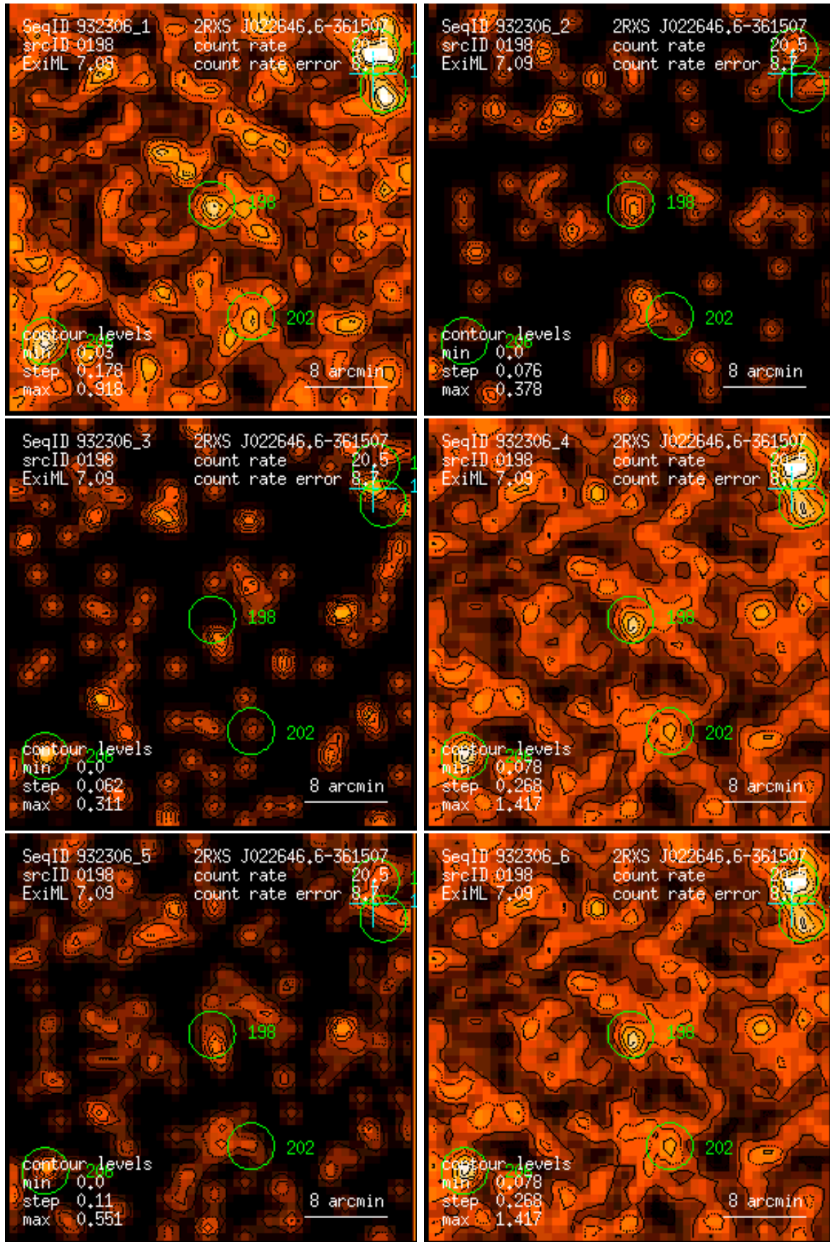
Figure 198: RASS 932306: detection 0198: band rate images, Gaussian filter: (1) PSPC channels 11 – 41, (2) 52 – 90, (3) 91 – 201, (4) 11 – 235, (5) 52 – 201, (6) 11 – 201. Broad band rates in counts/ks. Band rate contour levels in counts/ks/arcmin 2 .
