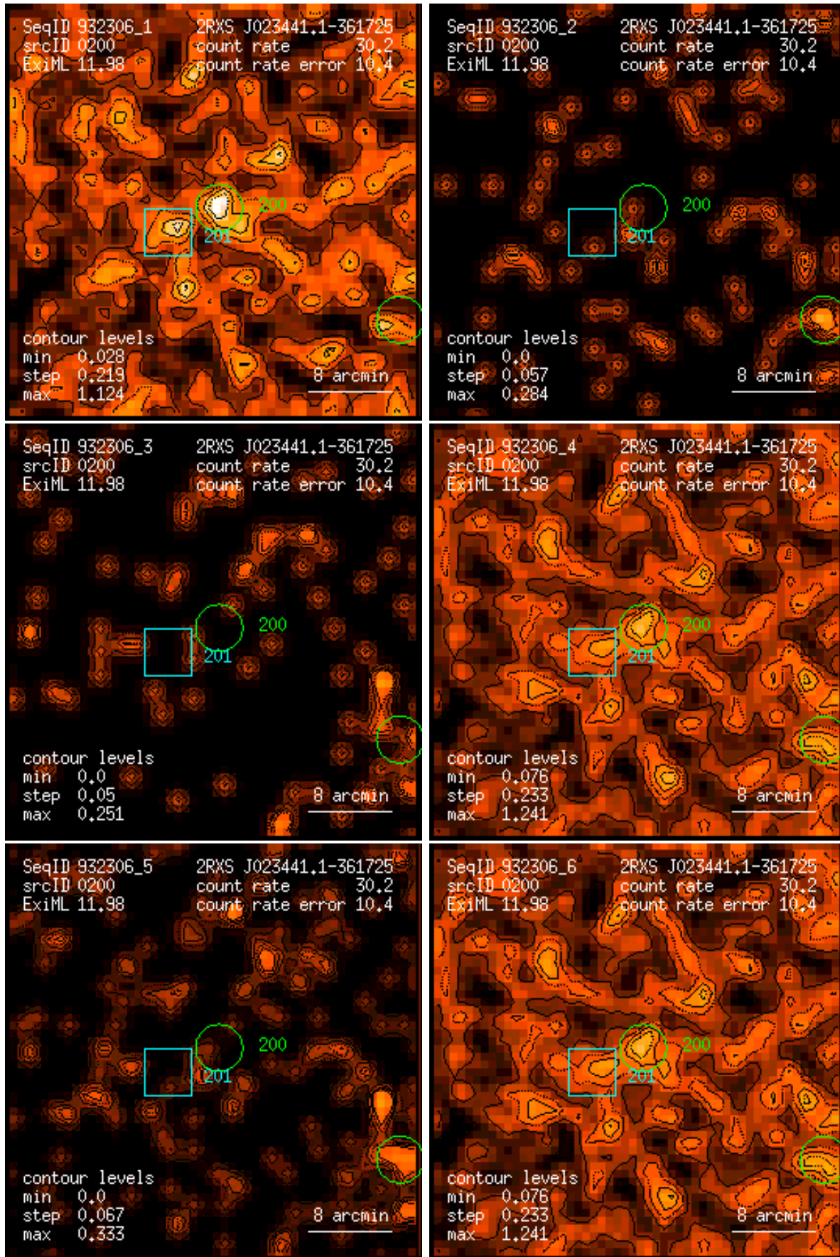
Figure 200: RASS 932306: detection 0200: band rate images, Gaussian filter: (1) PSPC channels 11 – 41, (2) 52 – 90, (3) 91 – 201, (4) 11 – 235, (5) 52 – 201, (6) 11 – 201. Broad band rates in counts/ks. Band rate contour levels in counts/ks/arcmin 2 .
