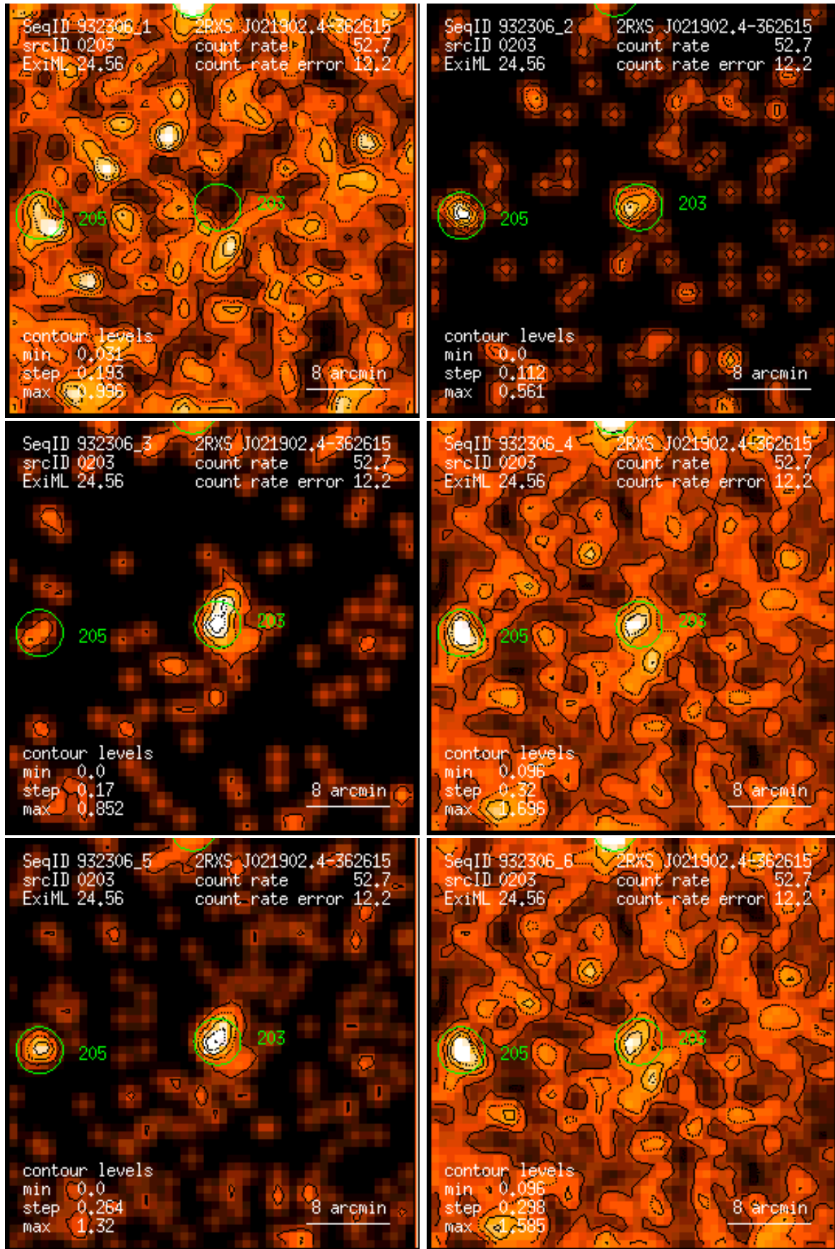
Figure 203: RASS 932306: detection 0203: band rate images, Gaussian filter: (1) PSPC channels 11 – 41, (2) 52 – 90, (3) 91 – 201, (4) 11 – 235, (5) 52 – 201, (6) 11 – 201. Broad band rates in counts/ks. Band rate contour levels in counts/ks/arcmin 2 .
