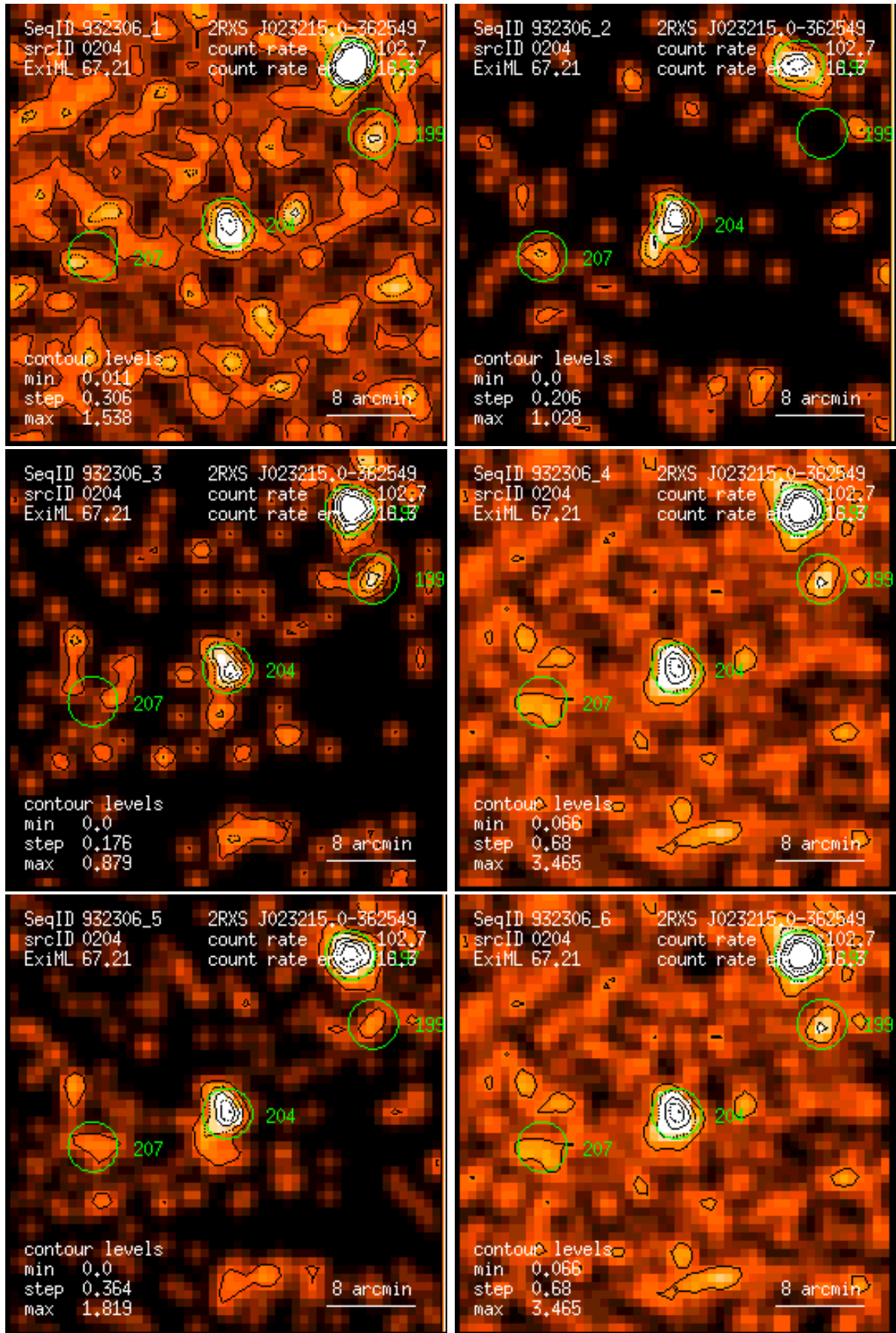
Figure 204: RASS 932306: detection 0204: band rate images, Gaussian filter: (1) PSPC channels 11 – 41, (2) 52 – 90, (3) 91 – 201, (4) 11 – 235, (5) 52 – 201, (6) 11 – 201. Broad band rates in counts/ks. Band rate contour levels in counts/ks/arcmin 2 .
