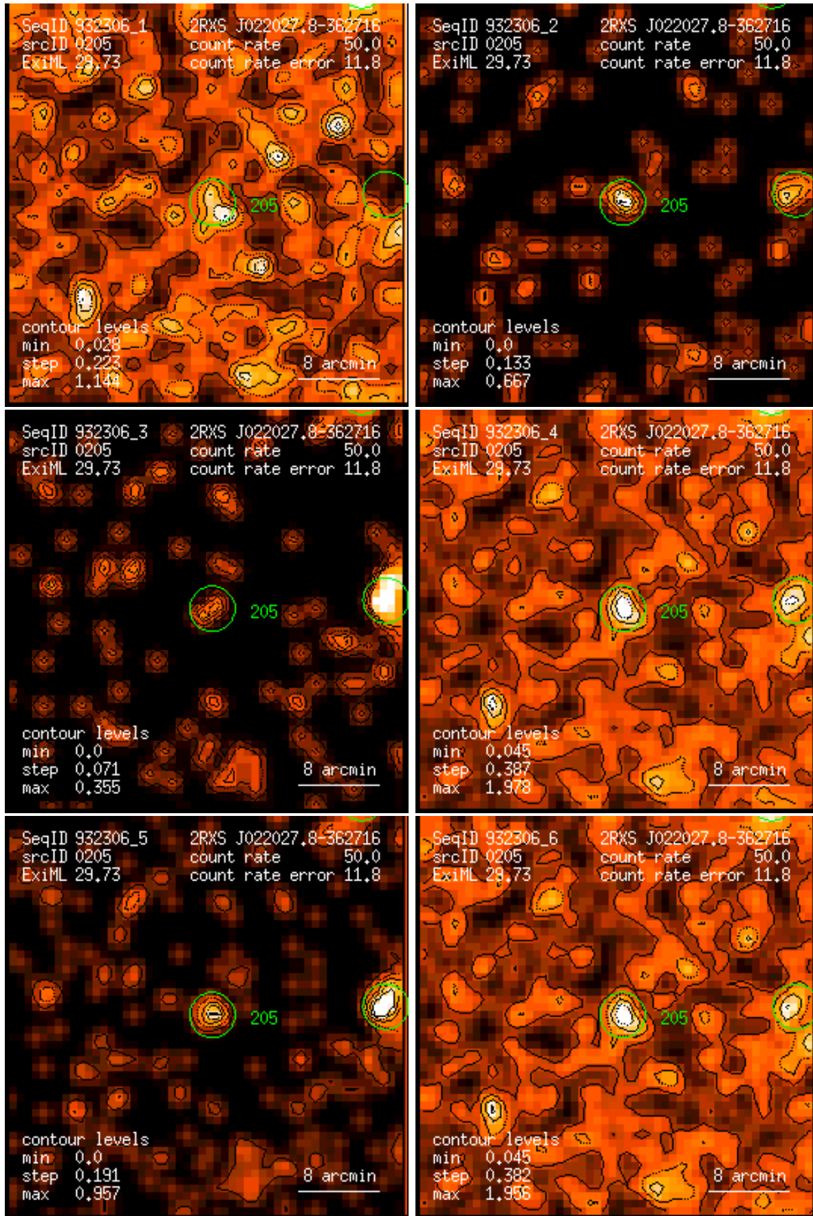
Figure 205: RASS 932306: detection 0205: band rate images, Gaussian filter: (1) PSPC channels 11 – 41, (2) 52 – 90, (3) 91 – 201, (4) 11 – 235, (5) 52 – 201, (6) 11 – 201. Broad band rates in counts/ks. Band rate contour levels in counts/ks/arcmin 2 .
