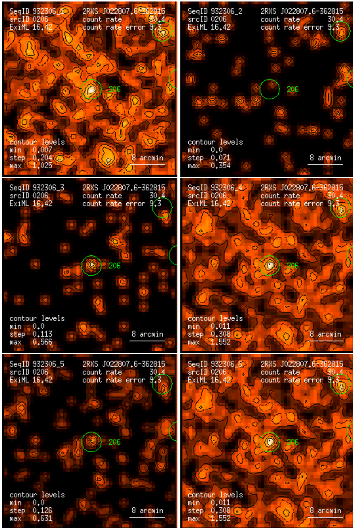
Figure 206: RASS 932306: detection 0206: band rate images, Gaussian filter: (1) PSPC channels 11 – 41, (2) 52 – 90, (3) 91 – 201, (4) 11 – 235, (5) 52 – 201, (6) 11 – 201. Broad band rates in counts/ks. Band rate contour levels in counts/ks/arcmin 2 .
