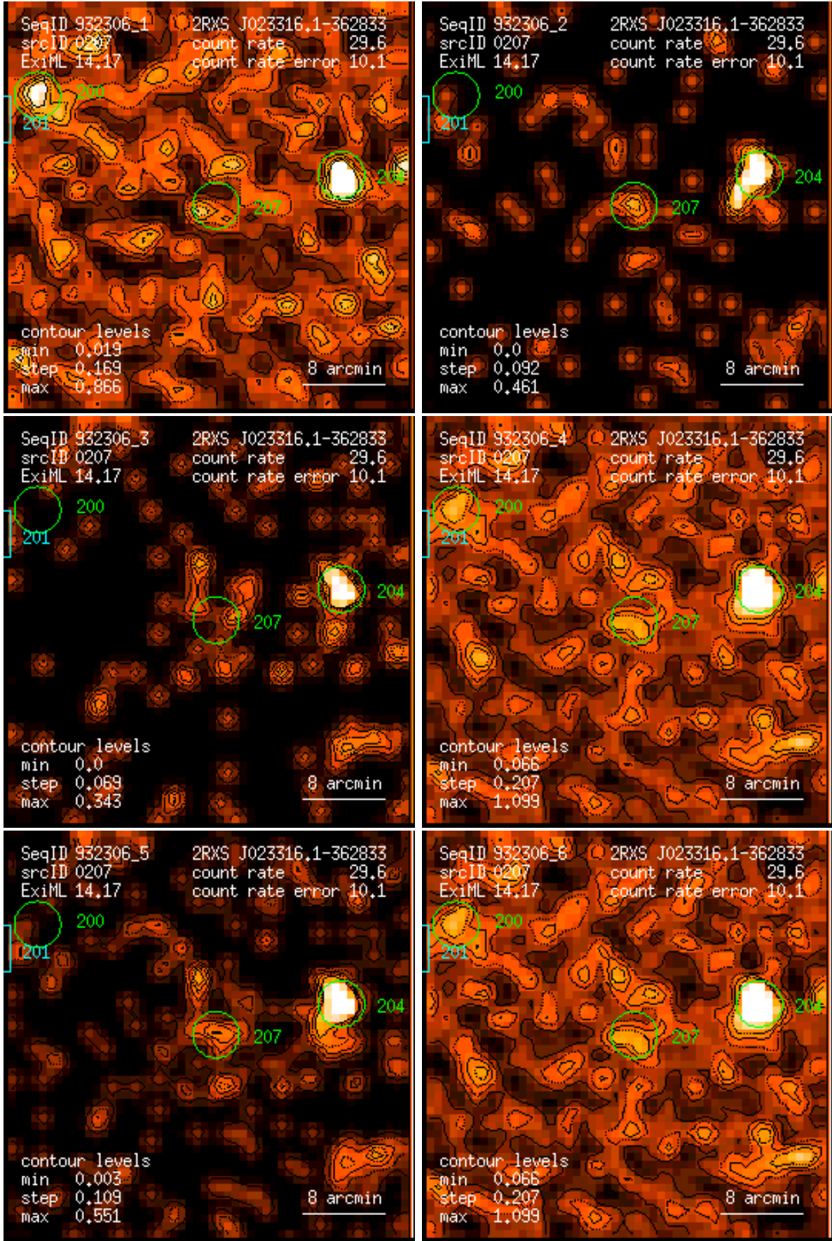
Figure 207: RASS 932306: detection 0207: band rate images, Gaussian filter: (1) PSPC channels 11 – 41, (2) 52 – 90, (3) 91 – 201, (4) 11 – 235, (5) 52 – 201, (6) 11 – 201. Broad band rates in counts/ks. Band rate contour levels in counts/ks/arcmin 2 .
