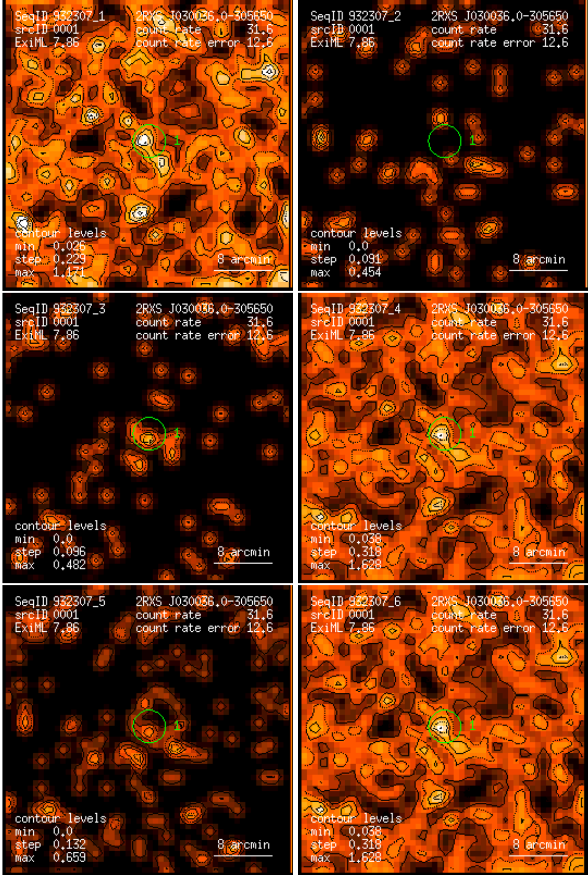
Figure 1: RASS 932307: detection 0001: band rate images, Gaussian filter: (1) PSPC channels 11 – 41, (2) 52 – 90, (3) 91 – 201, (4) 11 – 235, (5) 52 – 201, (6) 11 – 201. Broad band rates in counts/ks. Band rate contour levels in counts/ks/arcmin 2 .
