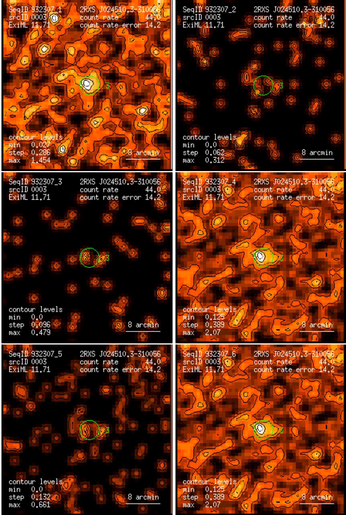
Figure 3: RASS 932307: detection 0003: band rate images, Gaussian filter: (1) PSPC channels 11 – 41, (2) 52 – 90, (3) 91 – 201, (4) 11 – 235, (5) 52 – 201, (6) 11 – 201. Broad band rates in counts/ks. Band rate contour levels in counts/ks/arcmin 2 .
