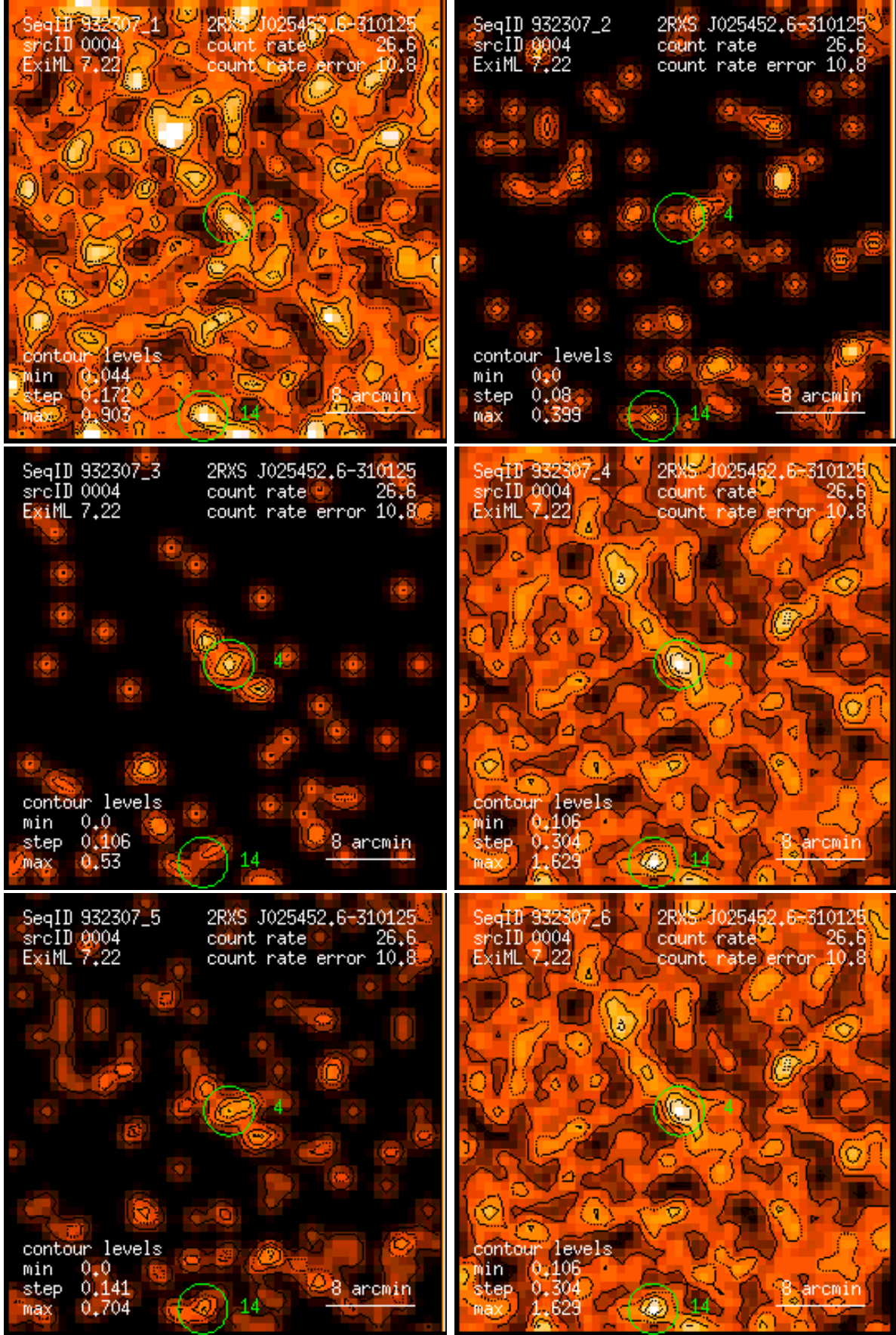
Figure 4: RASS 932307: detection 0004: band rate images, Gaussian filter: (1) PSPC channels 11 – 41, (2) 52 – 90, (3) 91 – 201, (4) 11 – 235, (5) 52 – 201, (6) 11 – 201. Broad band rates in counts/ks. Band rate contour levels in counts/ks/arcmin 2 .
