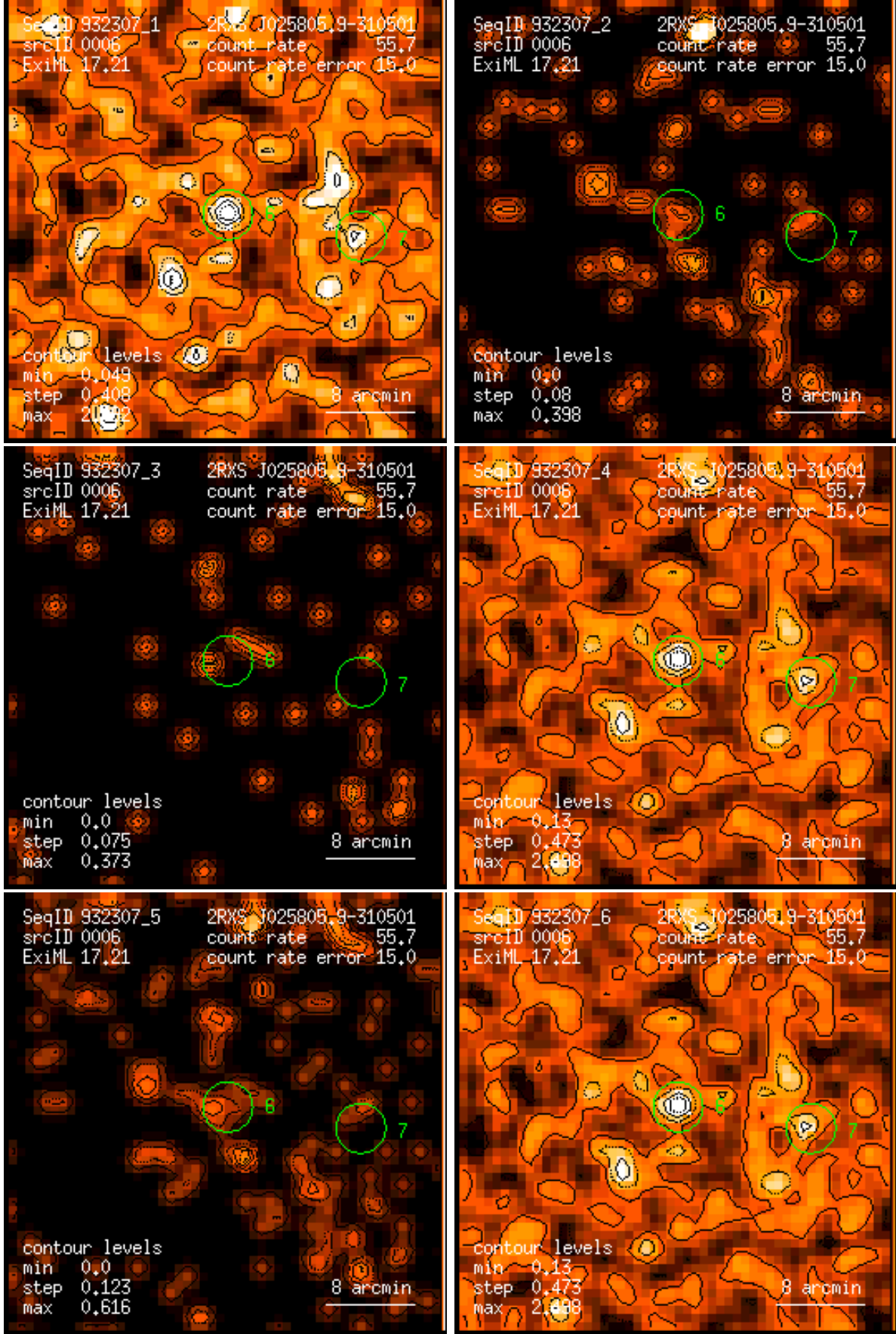
Figure 6: RASS 932307: detection 0006: band rate images, Gaussian filter: (1) PSPC channels 11 – 41, (2) 52 – 90, (3) 91 – 201, (4) 11 – 235, (5) 52 – 201, (6) 11 – 201. Broad band rates in counts/ks. Band rate contour levels in counts/ks/arcmin 2 .
