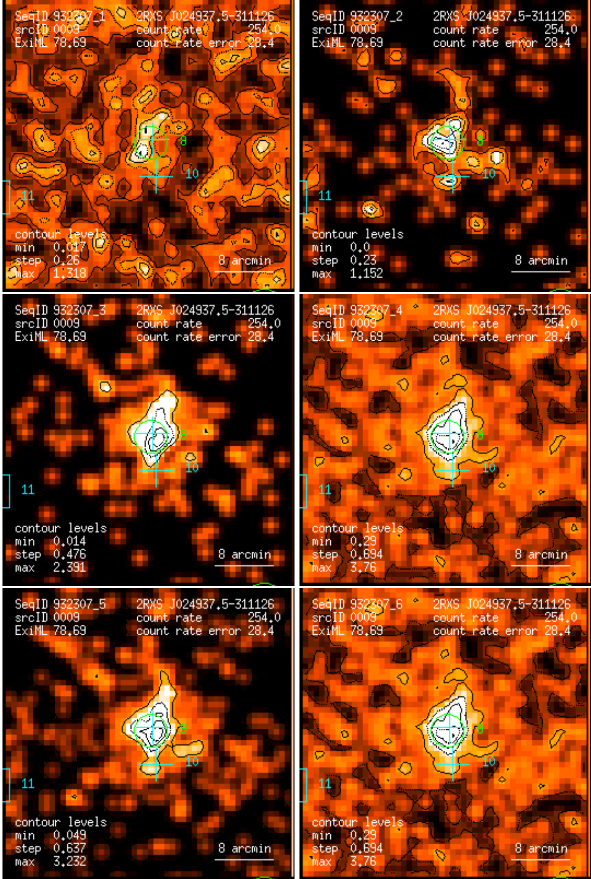
Figure 9: RASS 932307: detection 0009: band rate images, Gaussian filter: (1) PSPC channels 11 – 41, (2) 52 – 90, (3) 91 – 201, (4) 11 – 235, (5) 52 – 201, (6) 11 – 201. Broad band rates in counts/ks. Band rate contour levels in counts/ks/arcmin 2 .
