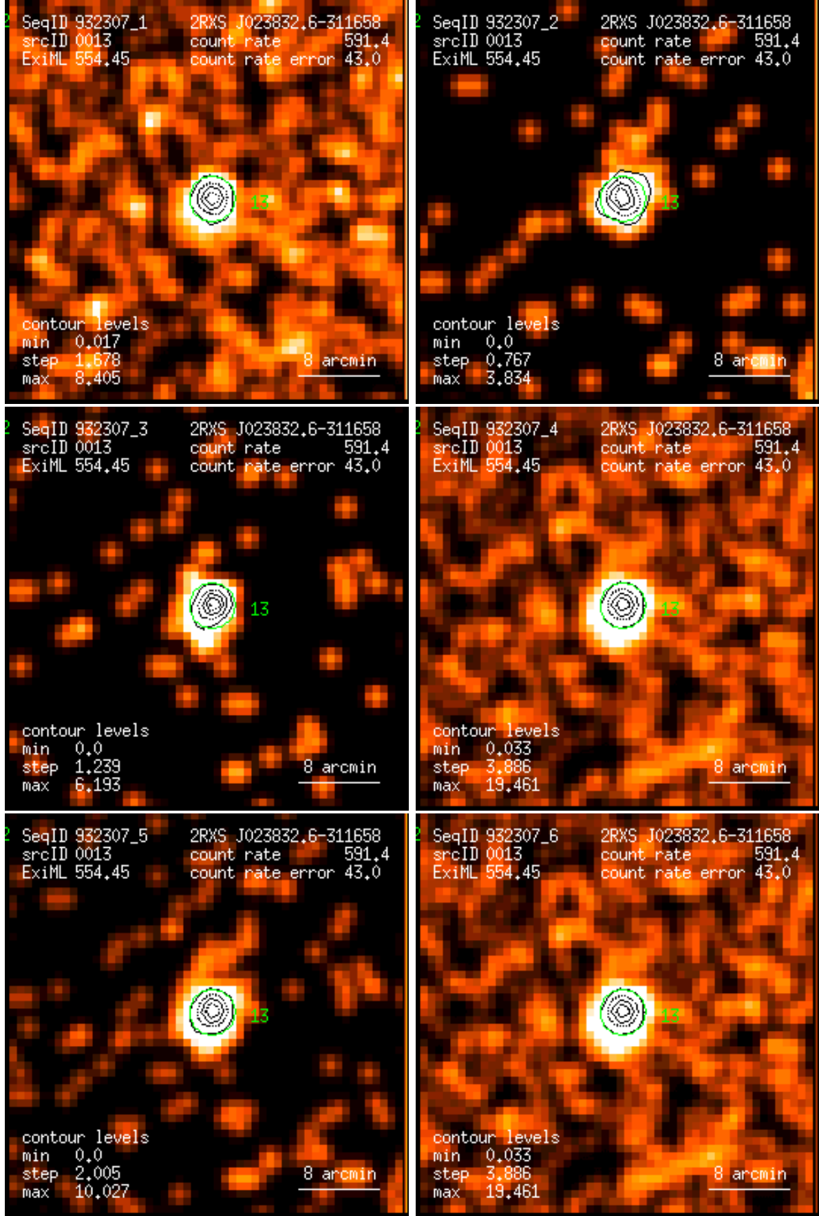
Figure 13: RASS 932307: detection 0013: band rate images, Gaussian filter: (1) PSPC channels 11 – 41, (2) 52 – 90, (3) 91 – 201, (4) 11 – 235, (5) 52 – 201, (6) 11 – 201. Broad band rates in counts/ks. Band rate contour levels in counts/ks/arcmin 2 .
