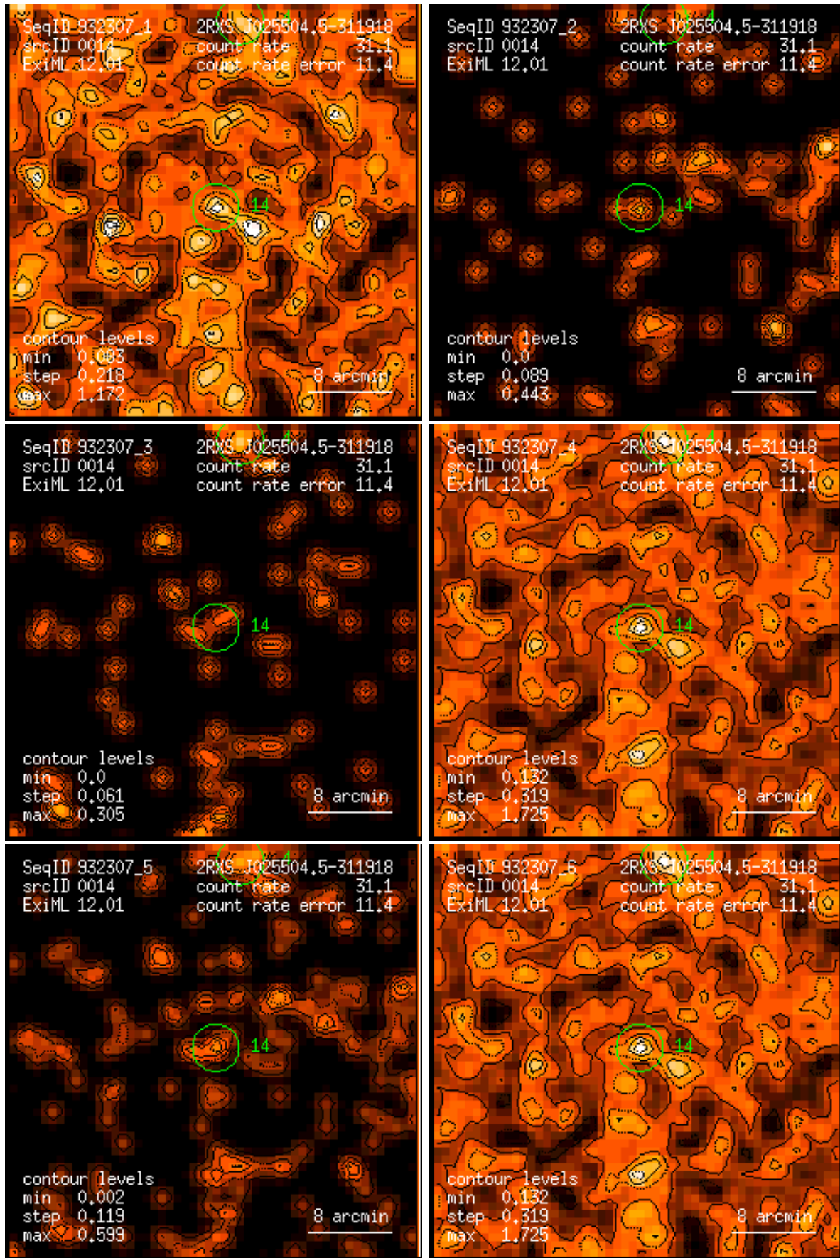
Figure 14: RASS 932307: detection 0014: band rate images, Gaussian filter: (1) PSPC channels 11 – 41, (2) 52 – 90, (3) 91 – 201, (4) 11 – 235, (5) 52 – 201, (6) 11 – 201. Broad band rates in counts/ks. Band rate contour levels in counts/ks/arcmin 2 .
