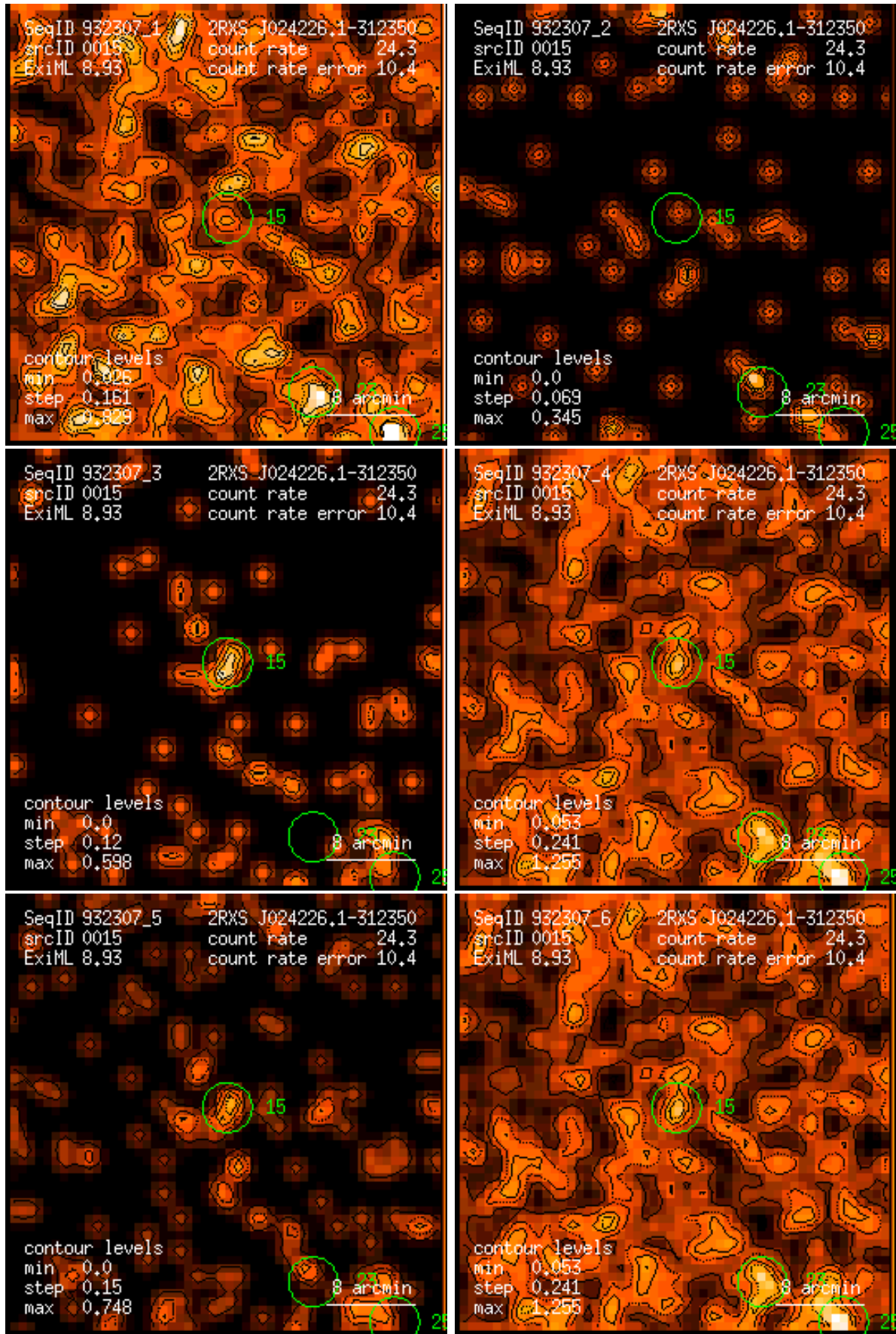
Figure 15: RASS 932307: detection 0015: band rate images, Gaussian filter: (1) PSPC channels 11 – 41, (2) 52 – 90, (3) 91 – 201, (4) 11 – 235, (5) 52 – 201, (6) 11 – 201. Broad band rates in counts/ks. Band rate contour levels in counts/ks/arcmin 2 .
