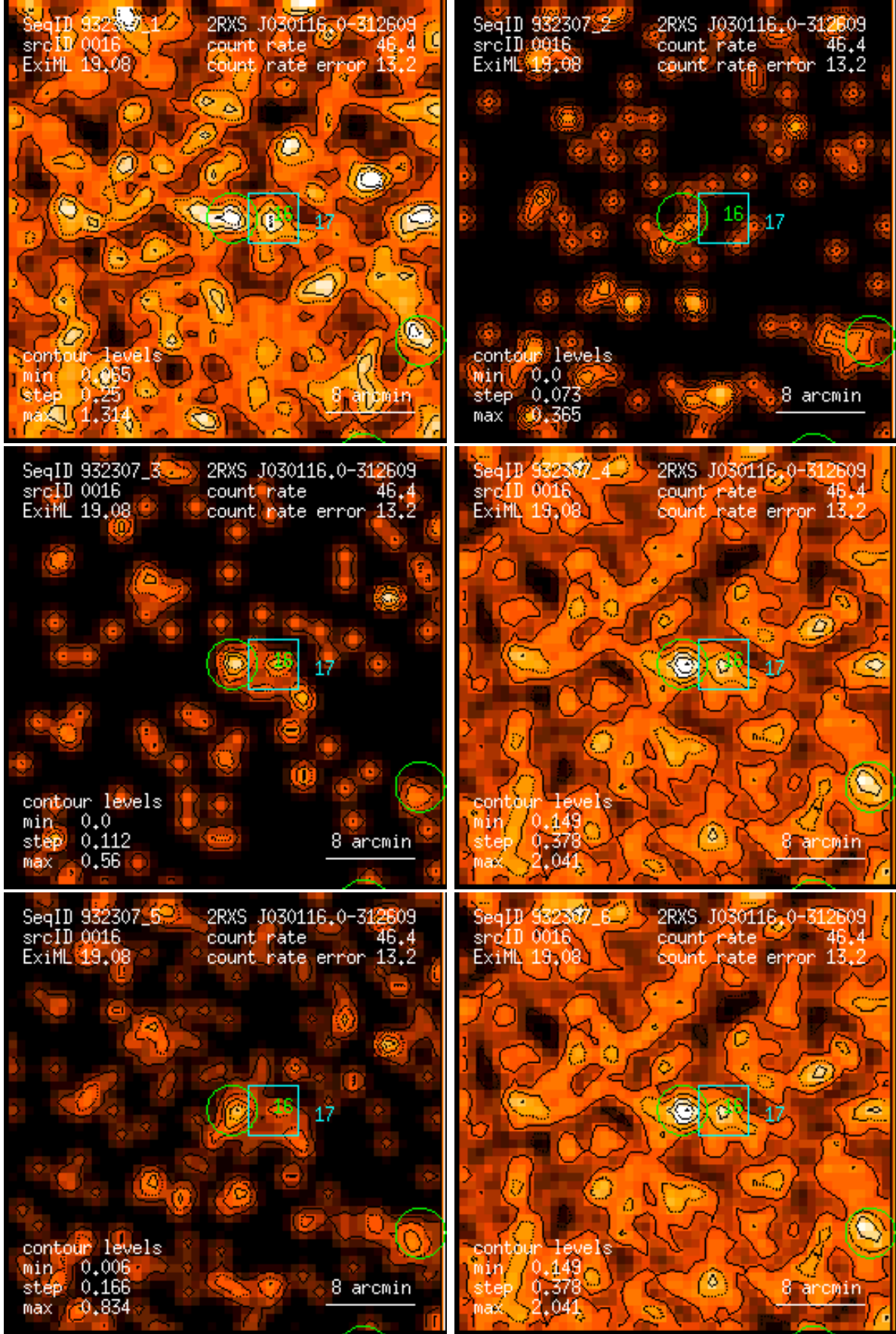
Figure 16: RASS 932307: detection 0016: band rate images, Gaussian filter: (1) PSPC channels 11 – 41, (2) 52 – 90, (3) 91 – 201, (4) 11 – 235, (5) 52 – 201, (6) 11 – 201. Broad band rates in counts/ks. Band rate contour levels in counts/ks/arcmin 2 .
