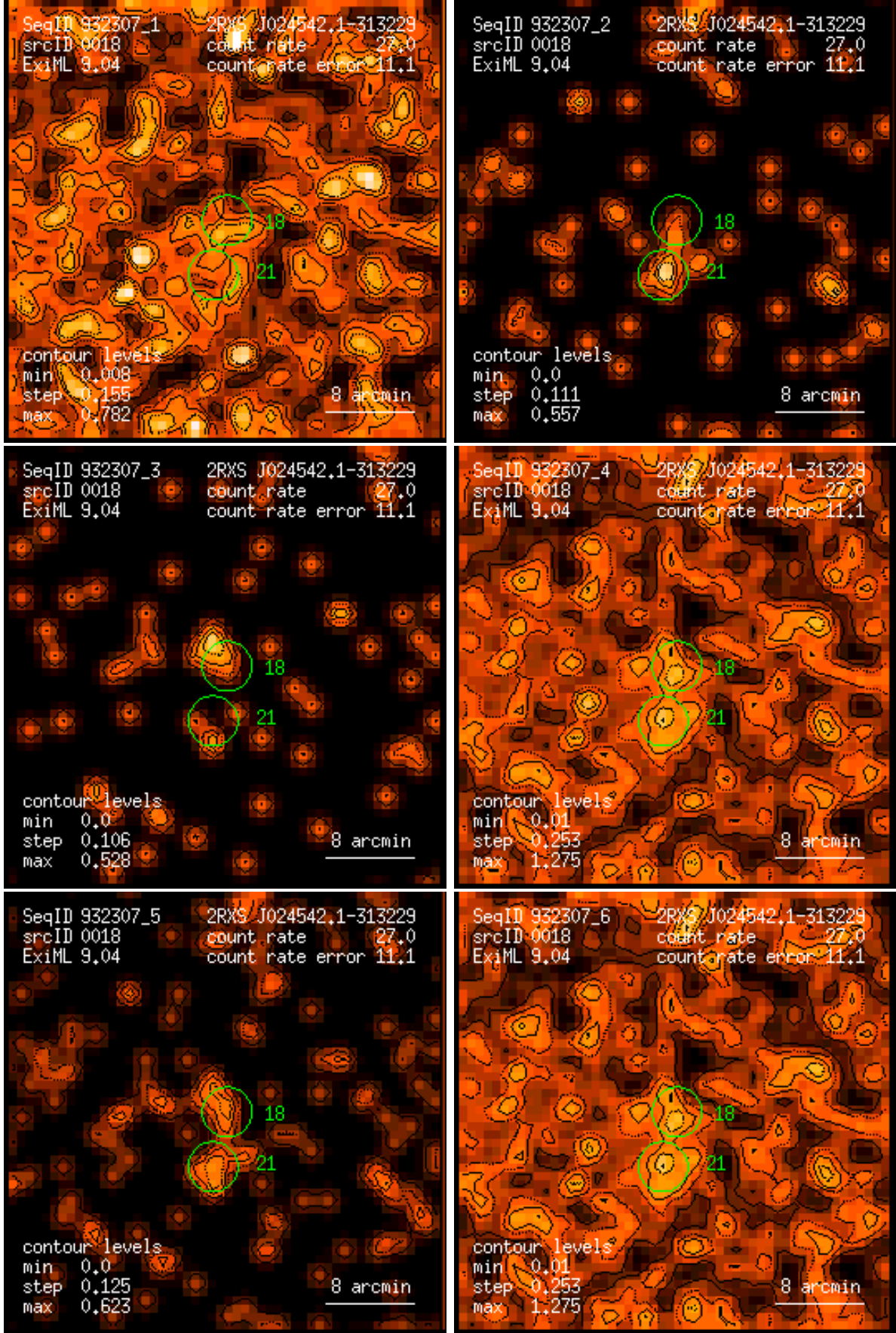
Figure 18: RASS 932307: detection 0018: band rate images, Gaussian filter: (1) PSPC channels 11 – 41, (2) 52 – 90, (3) 91 – 201, (4) 11 – 235, (5) 52 – 201, (6) 11 – 201. Broad band rates in counts/ks. Band rate contour levels in counts/ks/arcmin 2 .
