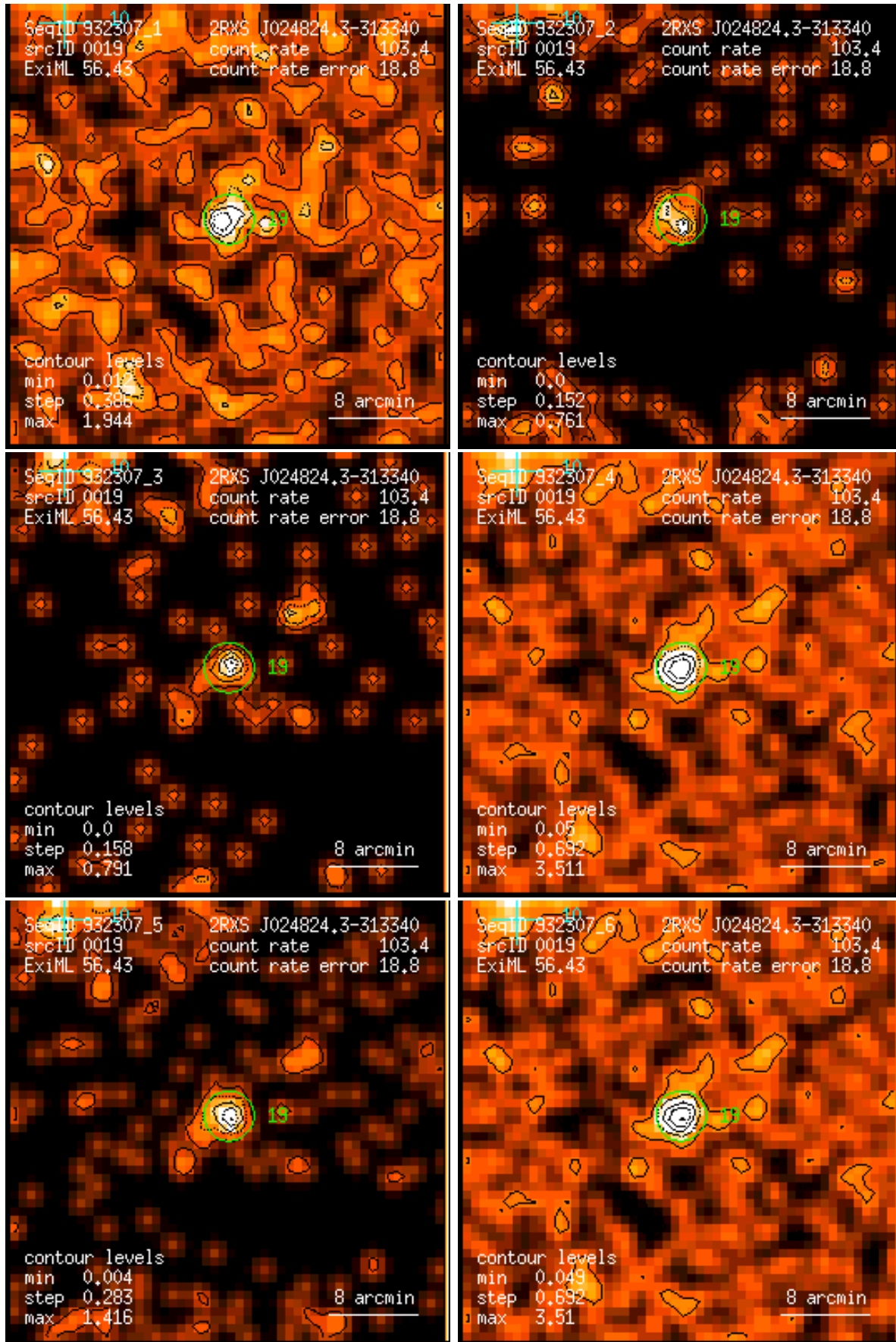
Figure 19: RASS 932307: detection 0019: band rate images, Gaussian filter: (1) PSPC channels 11 – 41, (2) 52 – 90, (3) 91 – 201, (4) 11 – 235, (5) 52 – 201, (6) 11 – 201. Broad band rates in counts/ks. Band rate contour levels in counts/ks/arcmin 2 .
