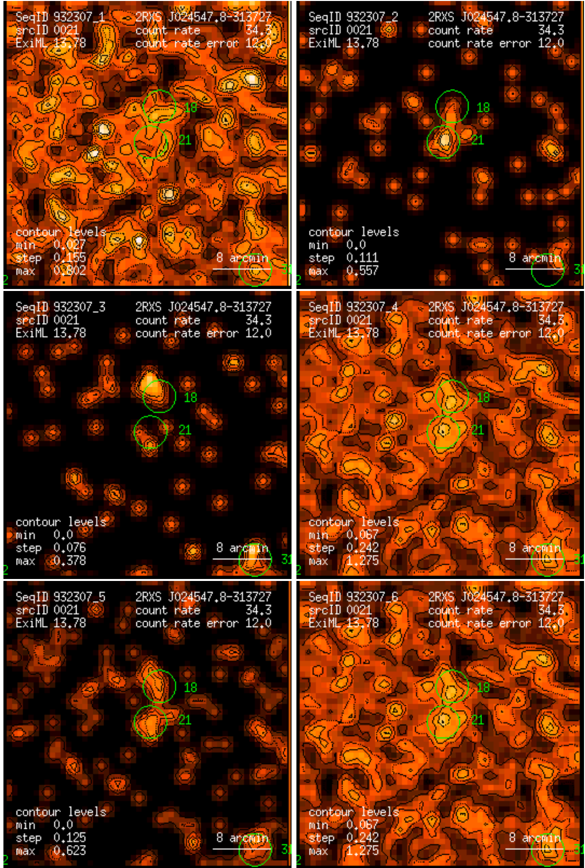
Figure 21: RASS 932307: detection 0021: band rate images, Gaussian filter: (1) PSPC channels 11 – 41, (2) 52 – 90, (3) 91 – 201, (4) 11 – 235, (5) 52 – 201, (6) 11 – 201. Broad band rates in counts/ks. Band rate contour levels in counts/ks/arcmin 2 .
