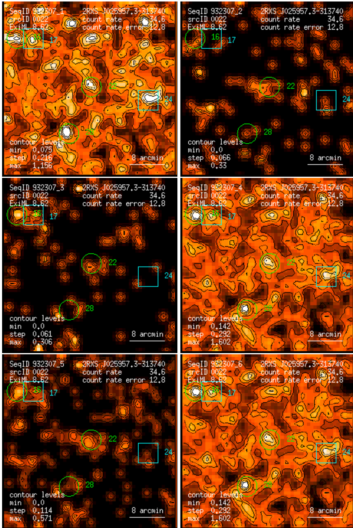
Figure 22: RASS 932307: detection 0022: band rate images, Gaussian filter: (1) PSPC channels 11 – 41, (2) 52 – 90, (3) 91 – 201, (4) 11 – 235, (5) 52 – 201, (6) 11 – 201. Broad band rates in counts/ks. Band rate contour levels in counts/ks/arcmin 2 .
