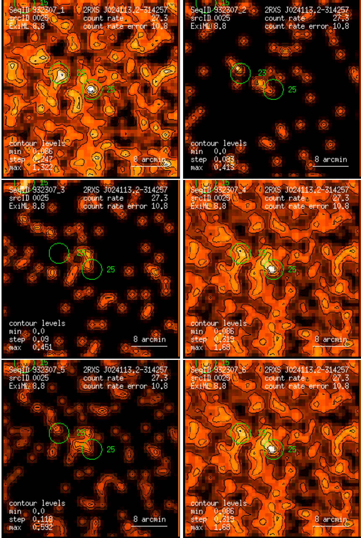
Figure 25: RASS 932307: detection 0025: band rate images, Gaussian filter: (1) PSPC channels 11 – 41, (2) 52 – 90, (3) 91 – 201, (4) 11 – 235, (5) 52 – 201, (6) 11 – 201. Broad band rates in counts/ks. Band rate contour levels in counts/ks/arcmin 2 .
