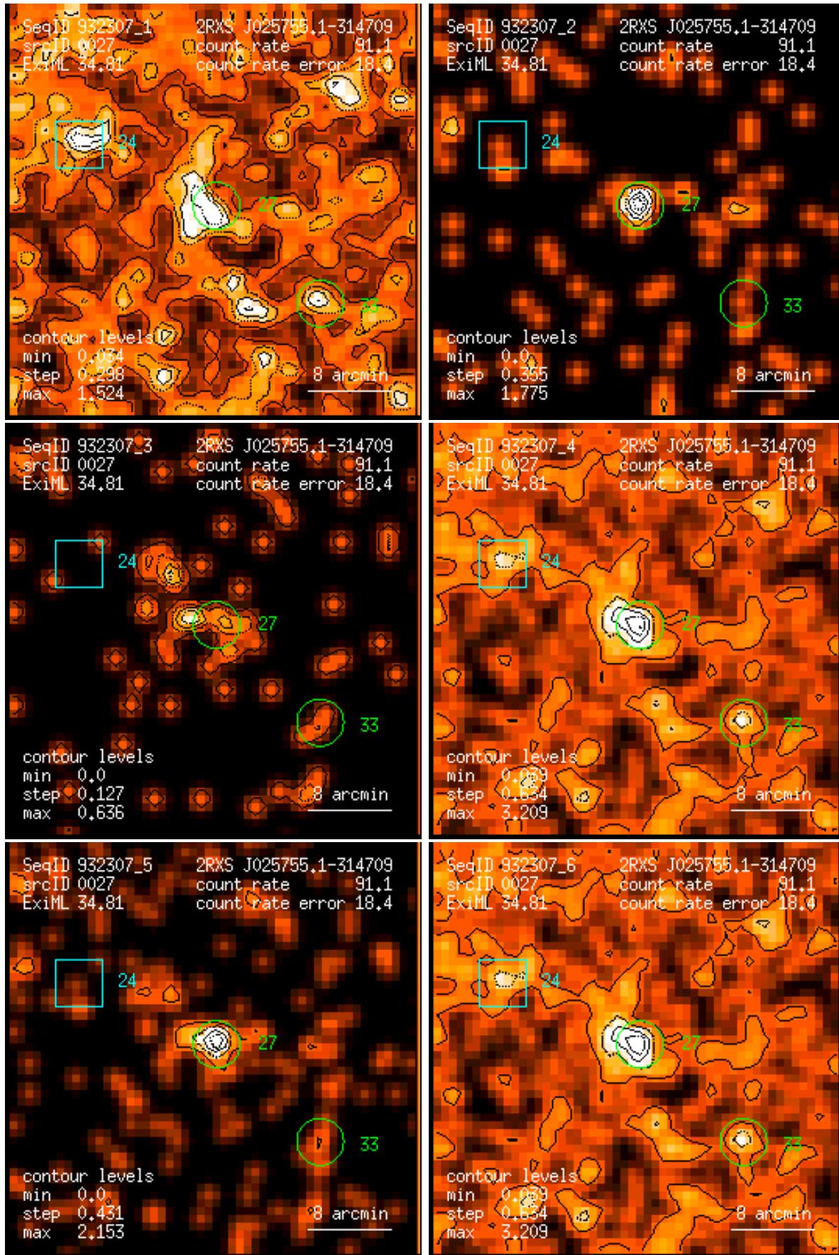
Figure 27: RASS 932307: detection 0027: band rate images, Gaussian filter: (1) PSPC channels 11 – 41, (2) 52 – 90, (3) 91 – 201, (4) 11 – 235, (5) 52 – 201, (6) 11 – 201. Broad band rates in counts/ks. Band rate contour levels in counts/ks/arcmin 2 .
