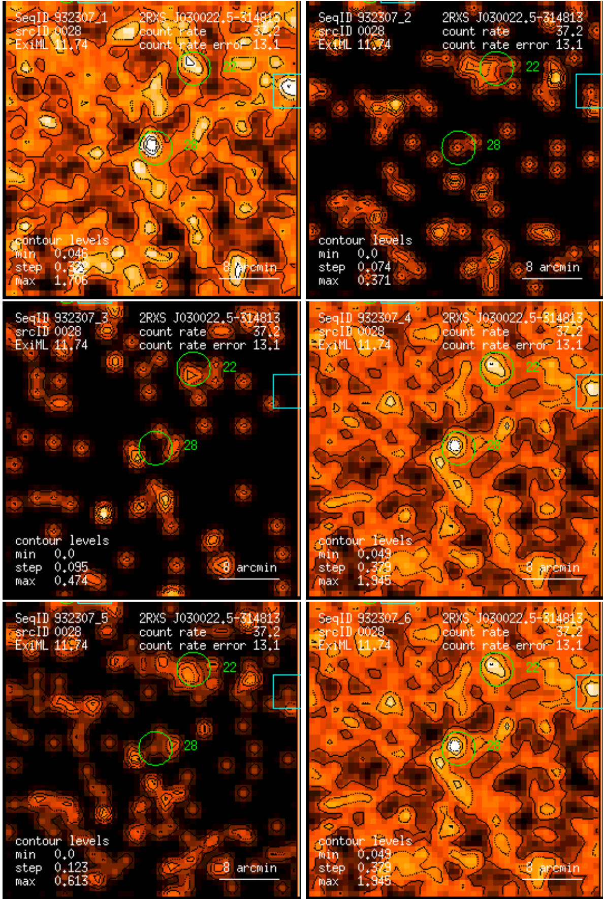
Figure 28: RASS 932307: detection 0028: band rate images, Gaussian filter: (1) PSPC channels 11 – 41, (2) 52 – 90, (3) 91 – 201, (4) 11 – 235, (5) 52 – 201, (6) 11 – 201. Broad band rates in counts/ks. Band rate contour levels in counts/ks/arcmin 2 .
