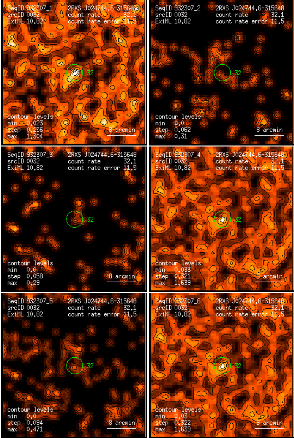
Figure 32: RASS 932307: detection 0032: band rate images, Gaussian filter: (1) PSPC channels 11 – 41, (2) 52 – 90, (3) 91 – 201, (4) 11 – 235, (5) 52 – 201, (6) 11 – 201. Broad band rates in counts/ks. Band rate contour levels in counts/ks/arcmin 2 .
