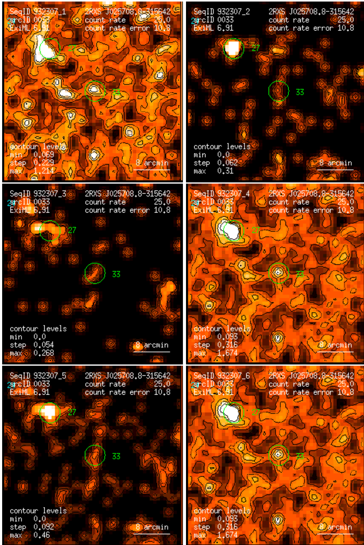
Figure 33: RASS 932307: detection 0033: band rate images, Gaussian filter: (1) PSPC channels 11 – 41, (2) 52 – 90, (3) 91 – 201, (4) 11 – 235, (5) 52 – 201, (6) 11 – 201. Broad band rates in counts/ks. Band rate contour levels in counts/ks/arcmin 2 .
