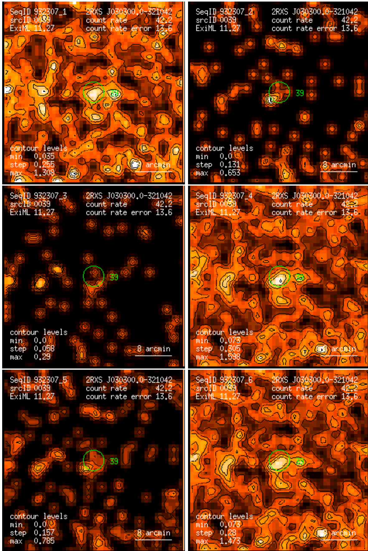
Figure 39: RASS 932307: detection 0039: band rate images, Gaussian filter: (1) PSPC channels 11 – 41, (2) 52 – 90, (3) 91 – 201, (4) 11 – 235, (5) 52 – 201, (6) 11 – 201. Broad band rates in counts/ks. Band rate contour levels in counts/ks/arcmin 2 .
