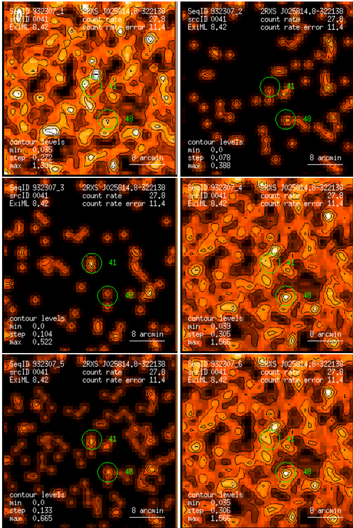
Figure 41: RASS 932307: detection 0041: band rate images, Gaussian filter: (1) PSPC channels 11 – 41, (2) 52 – 90, (3) 91 – 201, (4) 11 – 235, (5) 52 – 201, (6) 11 – 201. Broad band rates in counts/ks. Band rate contour levels in counts/ks/arcmin 2 .
