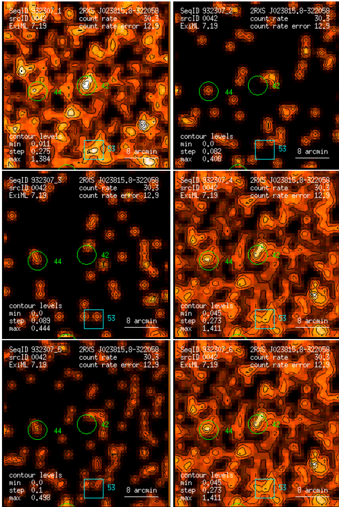
Figure 42: RASS 932307: detection 0042: band rate images, Gaussian filter: (1) PSPC channels 11 – 41, (2) 52 – 90, (3) 91 – 201, (4) 11 – 235, (5) 52 – 201, (6) 11 – 201. Broad band rates in counts/ks. Band rate contour levels in counts/ks/arcmin 2 .
