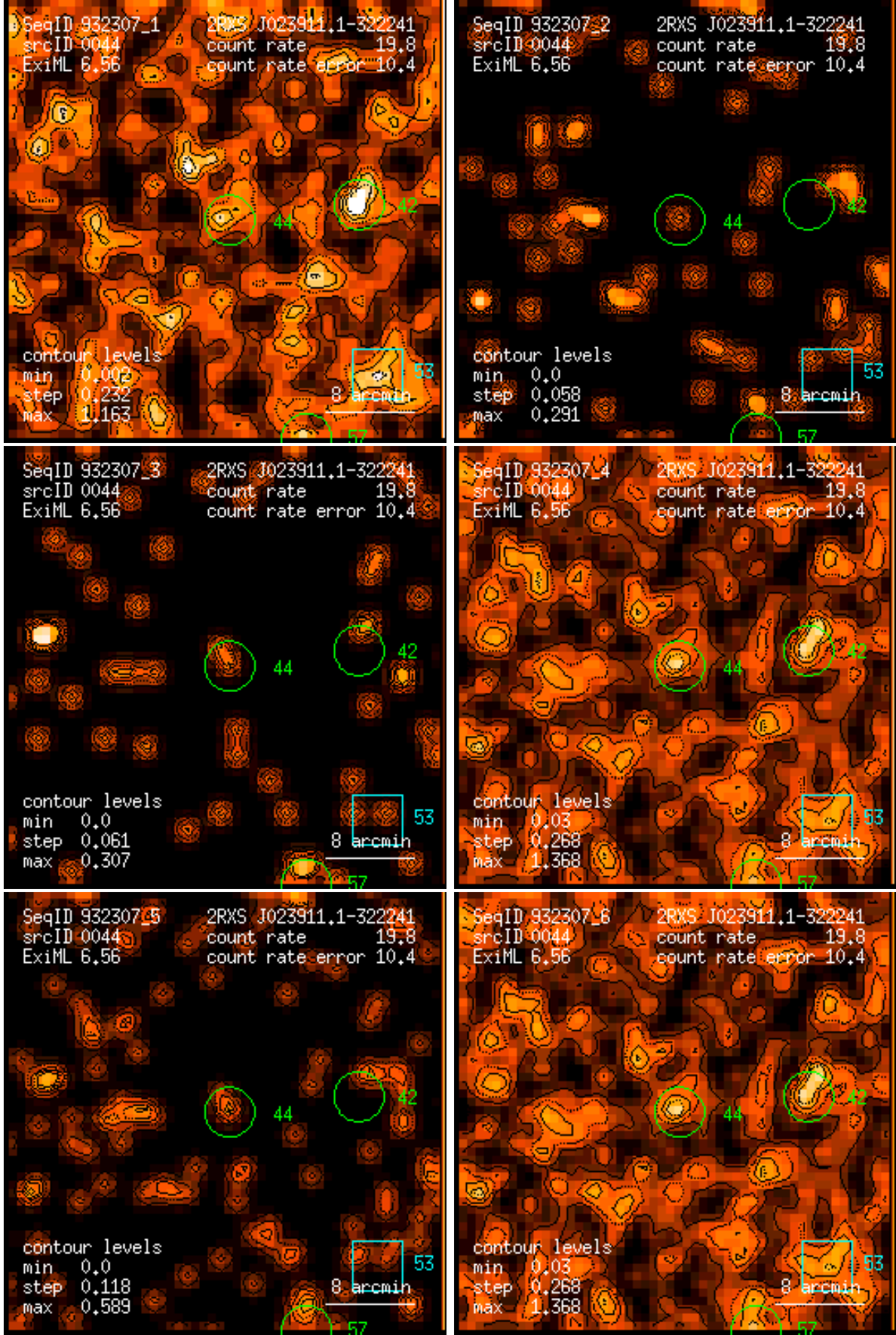
Figure 44: RASS 932307: detection 0044: band rate images, Gaussian filter: (1) PSPC channels 11 – 41, (2) 52 – 90, (3) 91 – 201, (4) 11 – 235, (5) 52 – 201, (6) 11 – 201. Broad band rates in counts/ks. Band rate contour levels in counts/ks/arcmin 2 .
