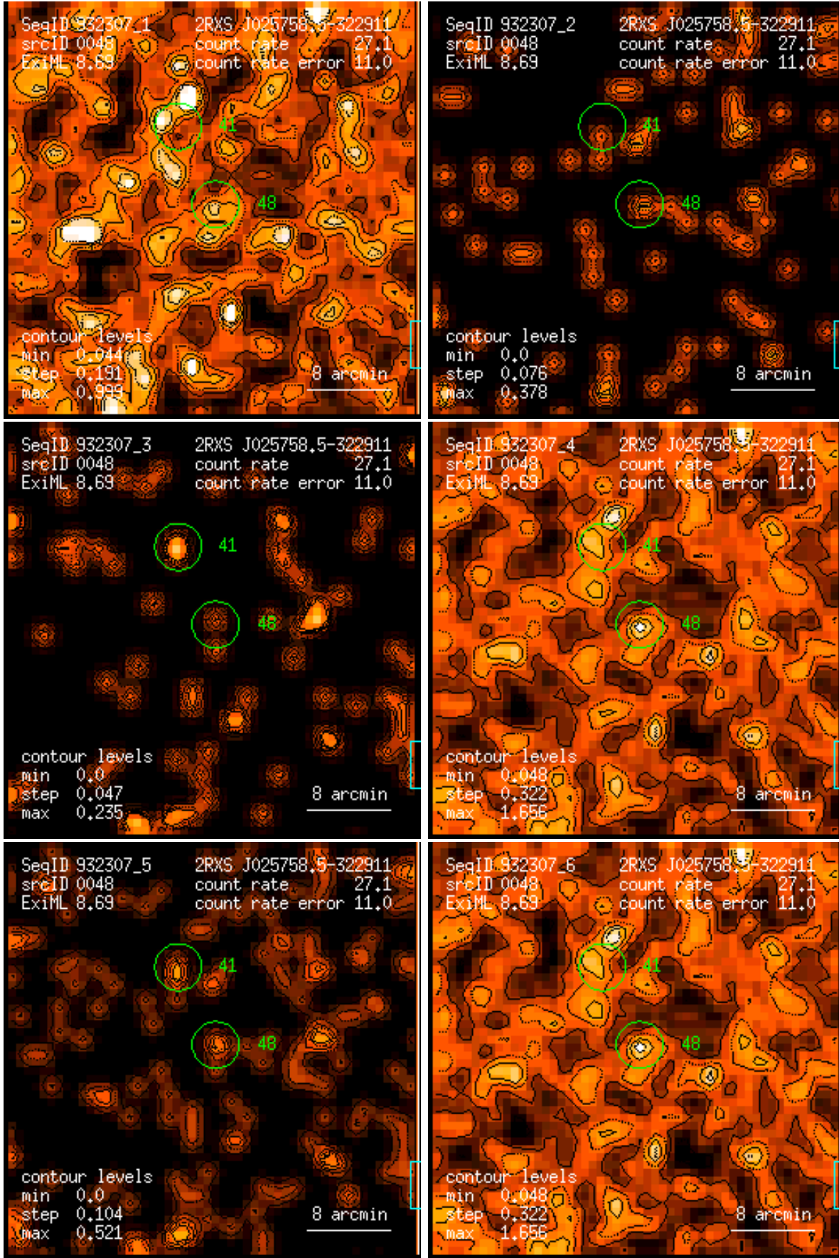
Figure 48: RASS 932307: detection 0048: band rate images, Gaussian filter: (1) PSPC channels 11 – 41, (2) 52 – 90, (3) 91 – 201, (4) 11 – 235, (5) 52 – 201, (6) 11 – 201. Broad band rates in counts/ks. Band rate contour levels in counts/ks/arcmin 2 .
