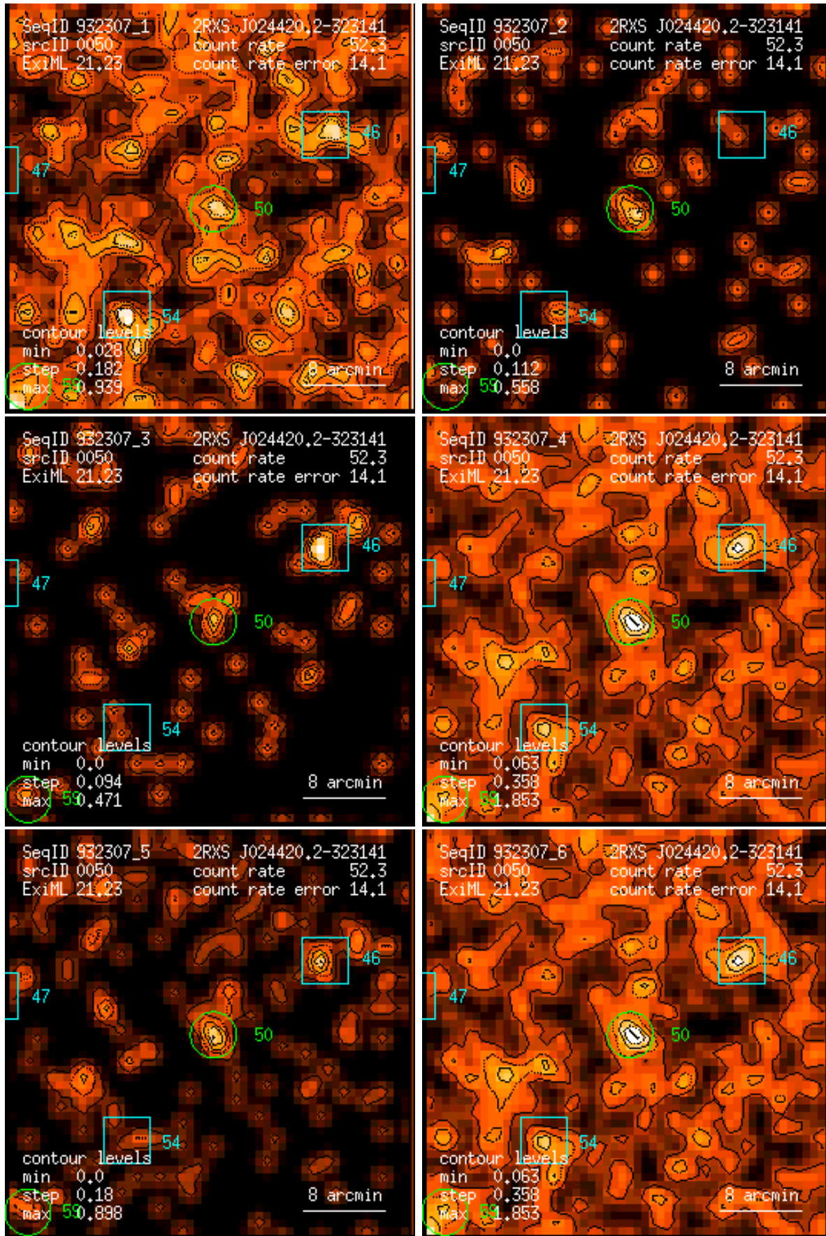
Figure 50: RASS 932307: detection 0050: band rate images, Gaussian filter: (1) PSPC channels 11 – 41, (2) 52 – 90, (3) 91 – 201, (4) 11 – 235, (5) 52 – 201, (6) 11 – 201. Broad band rates in counts/ks. Band rate contour levels in counts/ks/arcmin 2 .
