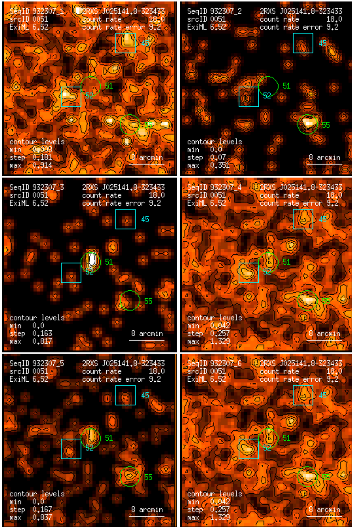
Figure 51: RASS 932307: detection 0051: band rate images, Gaussian filter: (1) PSPC channels 11 – 41, (2) 52 – 90, (3) 91 – 201, (4) 11 – 235, (5) 52 – 201, (6) 11 – 201. Broad band rates in counts/ks. Band rate contour levels in counts/ks/arcmin 2 .
