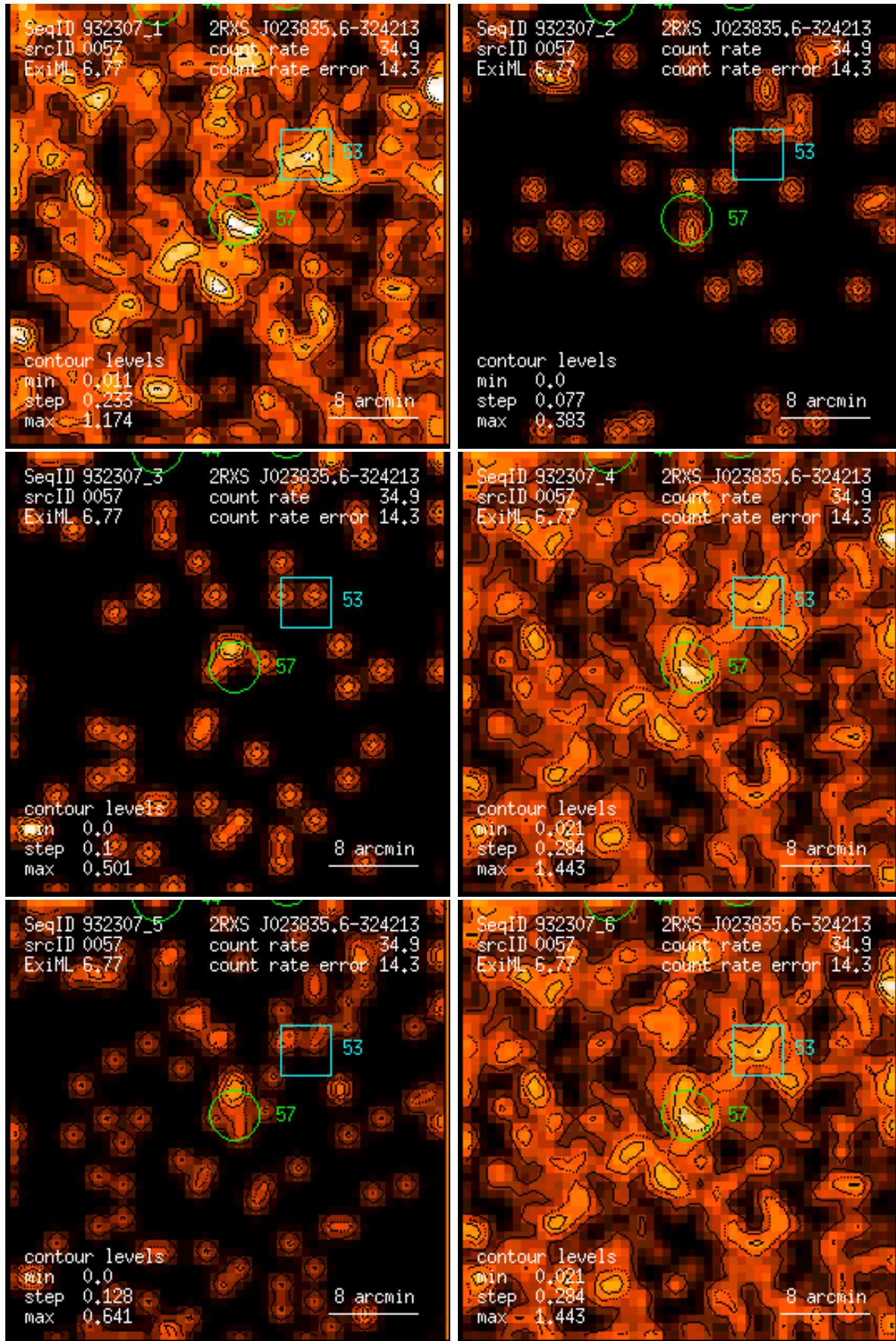
Figure 57: RASS 932307: detection 0057: band rate images, Gaussian filter: (1) PSPC channels 11 – 41, (2) 52 – 90, (3) 91 – 201, (4) 11 – 235, (5) 52 – 201, (6) 11 – 201. Broad band rates in counts/ks. Band rate contour levels in counts/ks/arcmin 2 .
