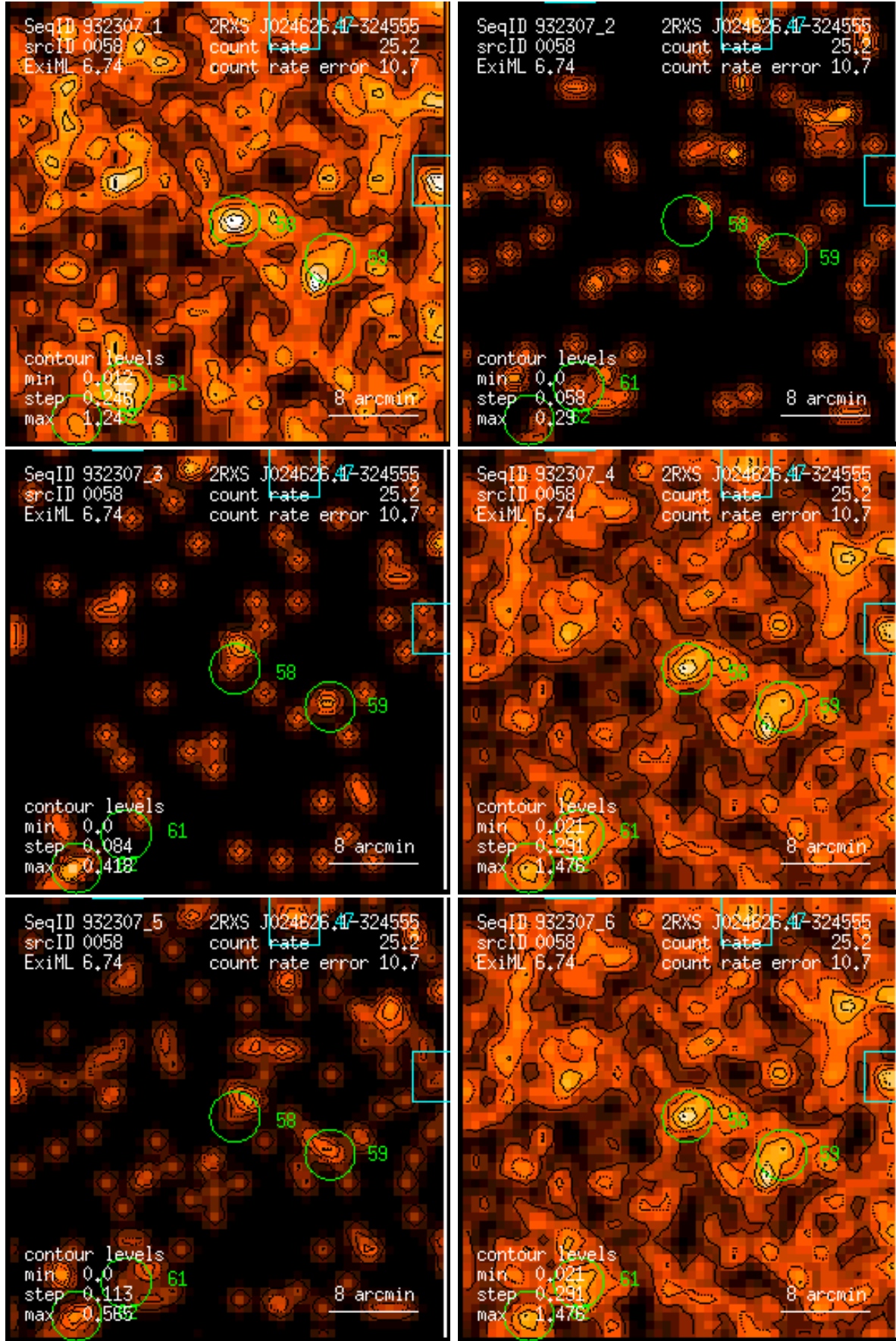
Figure 58: RASS 932307: detection 0058: band rate images, Gaussian filter: (1) PSPC channels 11 – 41, (2) 52 – 90, (3) 91 – 201, (4) 11 – 235, (5) 52 – 201, (6) 11 – 201. Broad band rates in counts/ks. Band rate contour levels in counts/ks/arcmin 2 .
