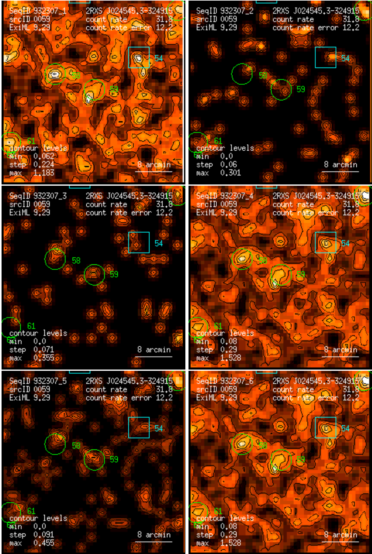
Figure 59: RASS 932307: detection 0059: band rate images, Gaussian filter: (1) PSPC channels 11 – 41, (2) 52 – 90, (3) 91 – 201, (4) 11 – 235, (5) 52 – 201, (6) 11 – 201. Broad band rates in counts/ks. Band rate contour levels in counts/ks/arcmin 2 .
