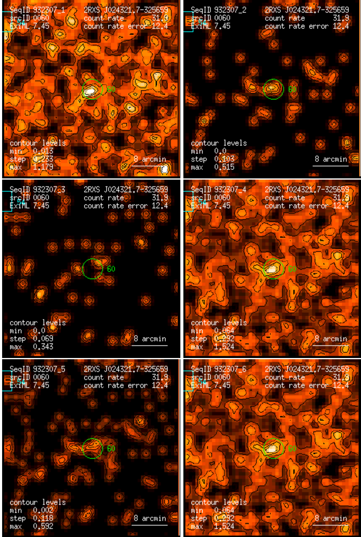
Figure 60: RASS 932307: detection 0060: band rate images, Gaussian filter: (1) PSPC channels 11 – 41, (2) 52 – 90, (3) 91 – 201, (4) 11 – 235, (5) 52 – 201, (6) 11 – 201. Broad band rates in counts/ks. Band rate contour levels in counts/ks/arcmin 2 .
