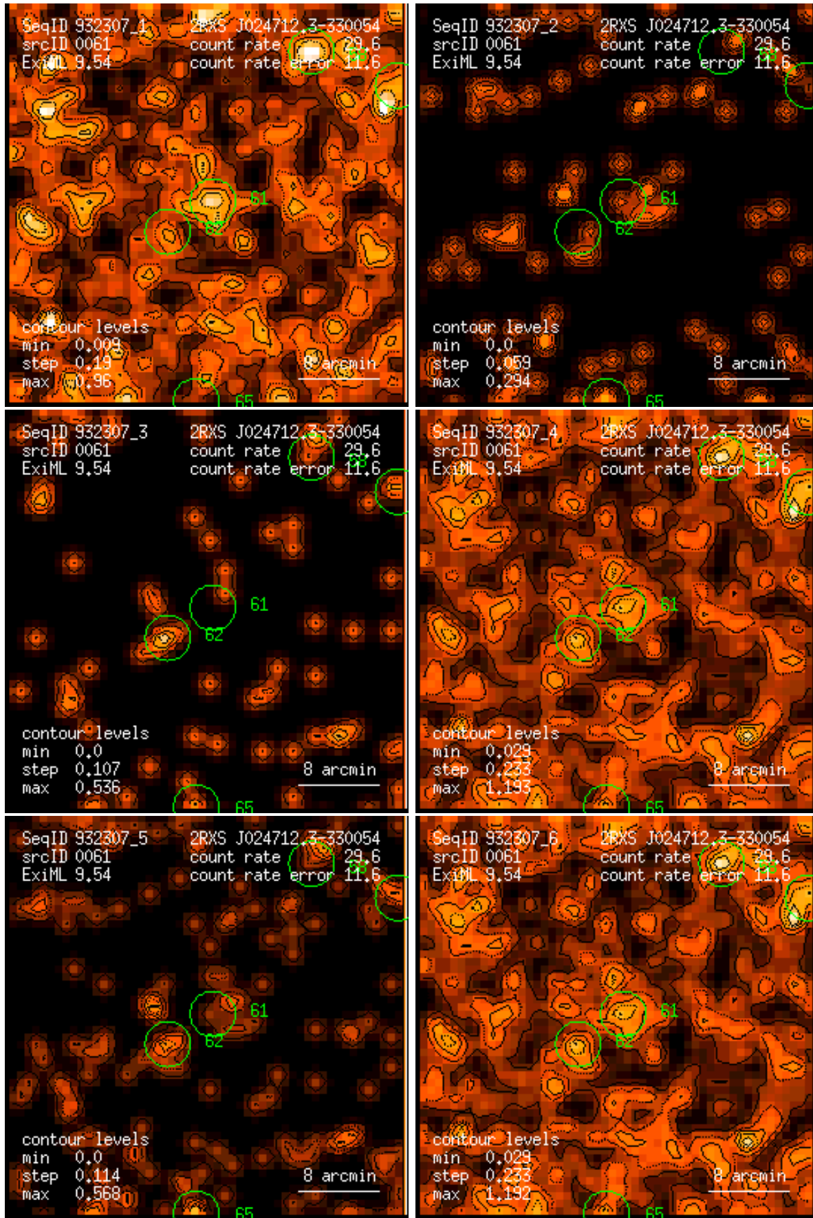
Figure 61: RASS 932307: detection 0061: band rate images, Gaussian filter: (1) PSPC channels 11 – 41, (2) 52 – 90, (3) 91 – 201, (4) 11 – 235, (5) 52 – 201, (6) 11 – 201. Broad band rates in counts/ks. Band rate contour levels in counts/ks/arcmin 2 .
